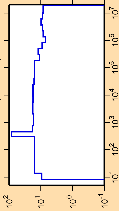
\Delta\sigma/\sigma vs. E for ^{106}\text{Pd}(n,\text{nonel.})
