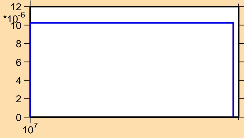
\sigma vs. E for ^{106}\text{Pd}(n,t)
