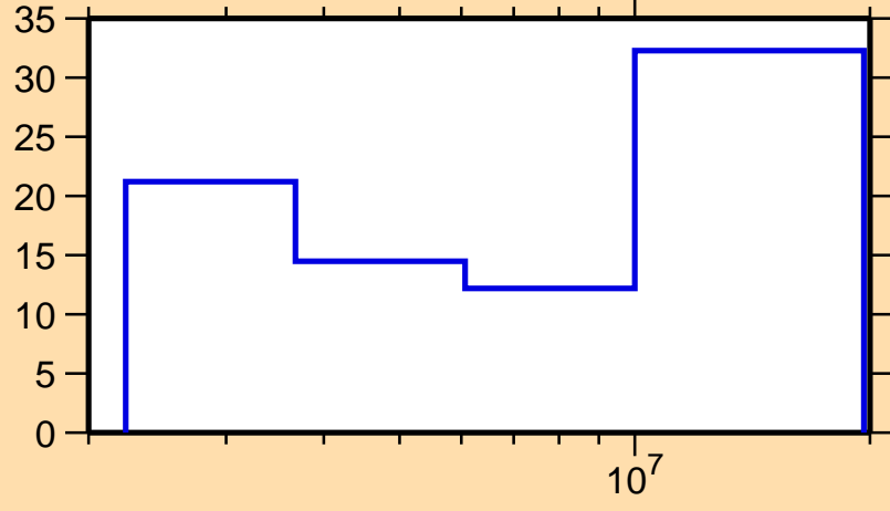
\Delta\sigma/\sigma vs. E for ^{106}\text{Pd}(n,n\text{cont.})
