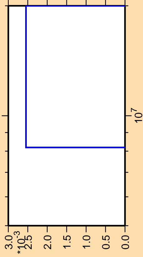
\Delta\sigma/\sigma vs. E for ^{106}\text{Pd}(n,\text{pd})
