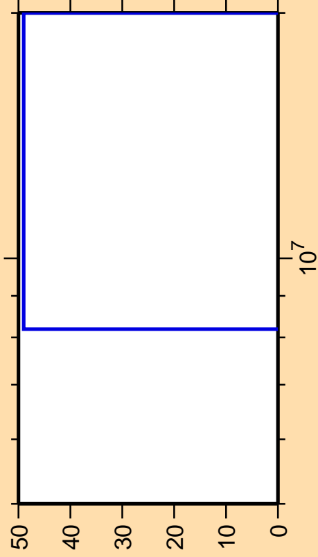
\Delta\sigma/\sigma vs. E for ^{106}\text{Pd}(n,np)
