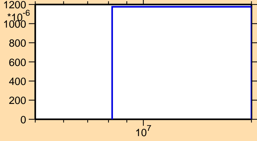
\sigma vs. E for ^{106}\text{Pd}(n,np)
