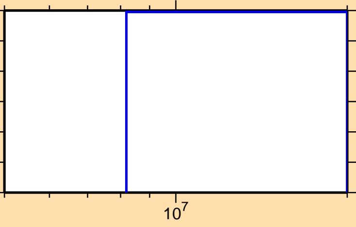
\sigma vs. E for ^{106}\text{Pd}(n,3n)
