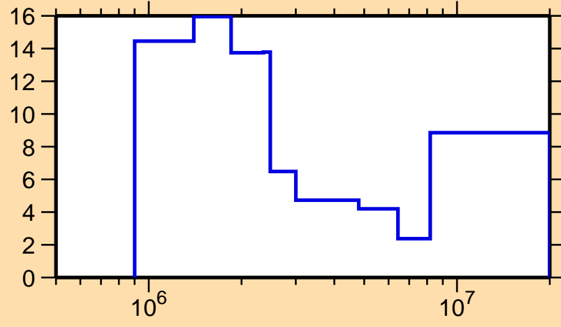
\Delta\sigma/\sigma vs. E for ^{106}\text{Pd}(n,\text{tot.})
