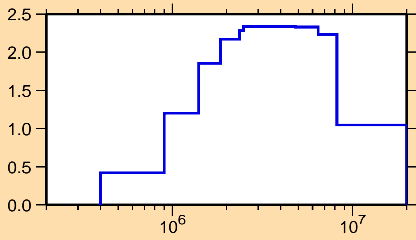
\sigma vs. E for ^{106}\text{Pd}(n,\text{inel.})
