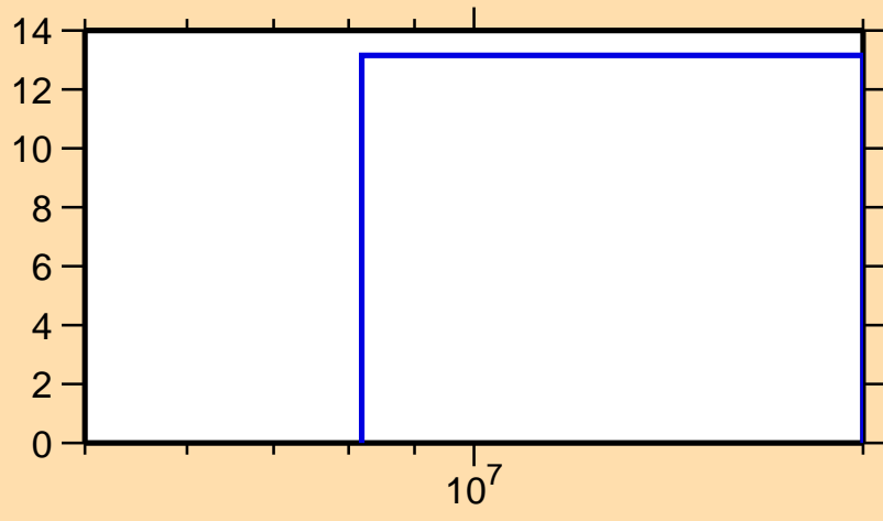
\Delta\sigma/\sigma vs. E for ^{106}\text{Pd}(n,2n)
