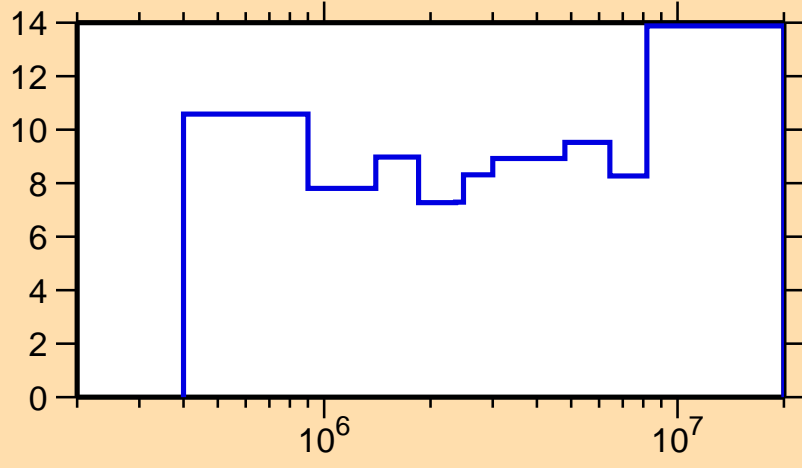
\Delta\sigma/\sigma vs. E for ^{106}\text{Pd}(n,\text{inel.})
