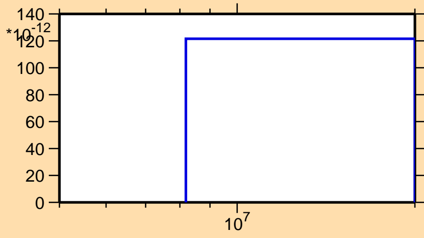
\sigma vs. E for ^{106}\text{Pd}(n,\text{nd})
