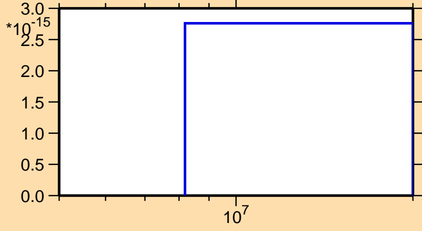
\sigma vs. E for ^{106}\text{Pd}(n,\text{pd})
