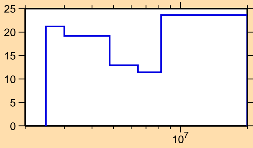
\Delta\sigma/\sigma vs. E for ^{106}\text{Pd}(n,n\text{cont.})
