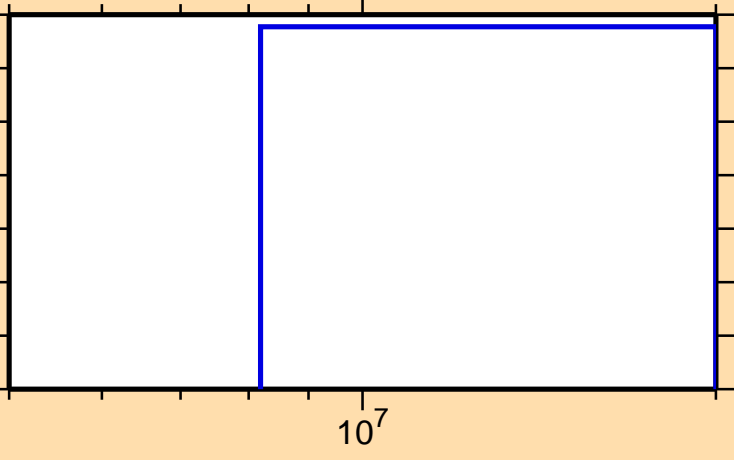
\sigma vs. E for ^{106}\text{Pd}(n,d)
