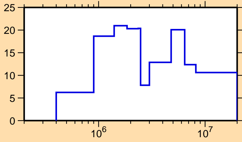
\Delta\sigma/\sigma vs. E for ^{106}\text{Pd}(n,\text{el.})
