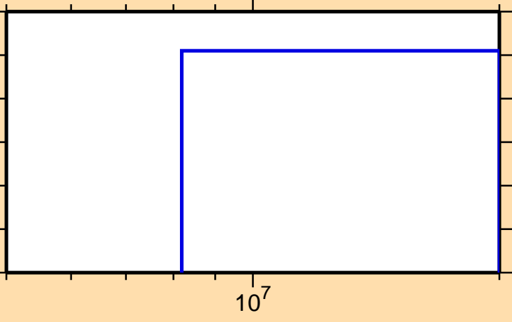
\sigma vs. E for ^{106}\text{Pd}(n,p\alpha)
