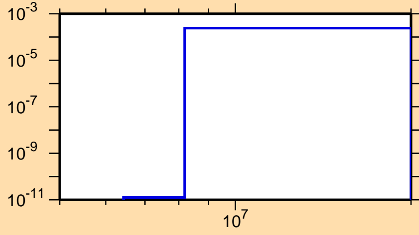
\sigma vs. E for ^{106}\text{Pd}(n,n\alpha)
