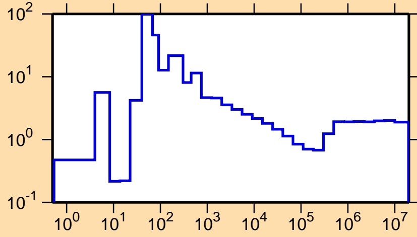
\sigma vs. E for ^{107}\text{Pd}(n,\text{nonel.})
