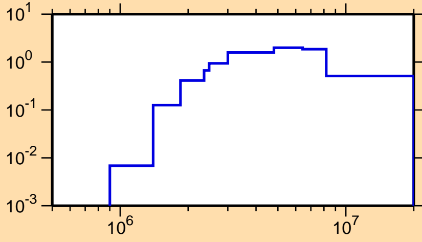
\sigma vs. E for ^{107}\text{Pd}(n,n\text{cont.})
