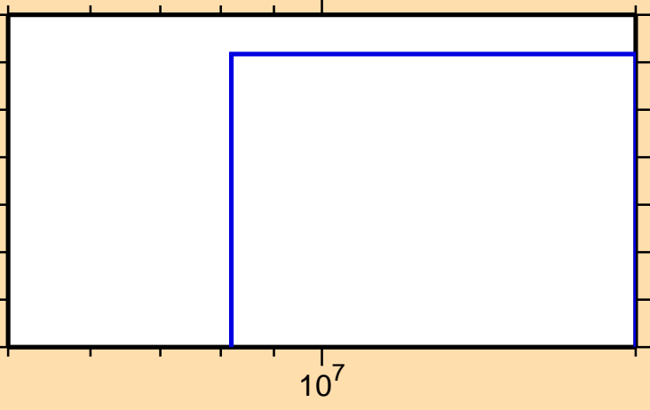
\sigma vs. E for ^{107}\text{Pd}(n,t)
