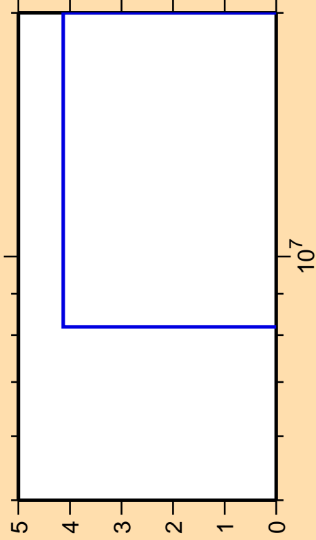
\Delta\sigma/\sigma vs. E for ^{107}\text{Pd}(n,nt)
