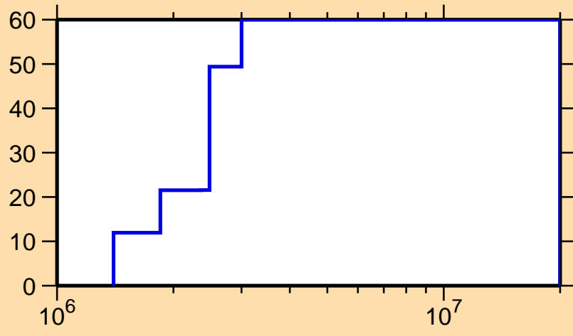
\Delta\sigma/\sigma vs. E for ^{107}\text{Pd}(n,n_1)
