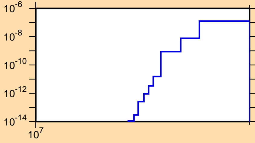
\sigma vs. E for ^{107}\text{Pd}(n,2n\alpha)
