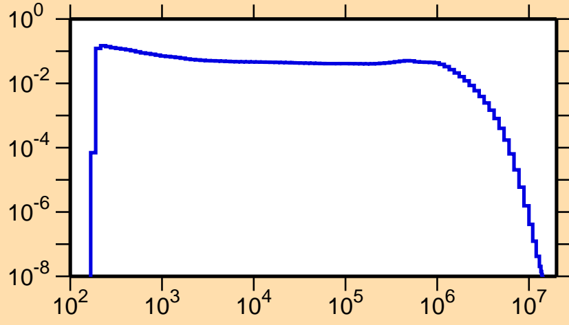
\sigma vs. E for ^{107}\text{Pd}(n,n_1)
