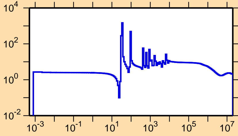
\sigma vs. E for ^{108}\text{Pd}(n,\text{el.})
