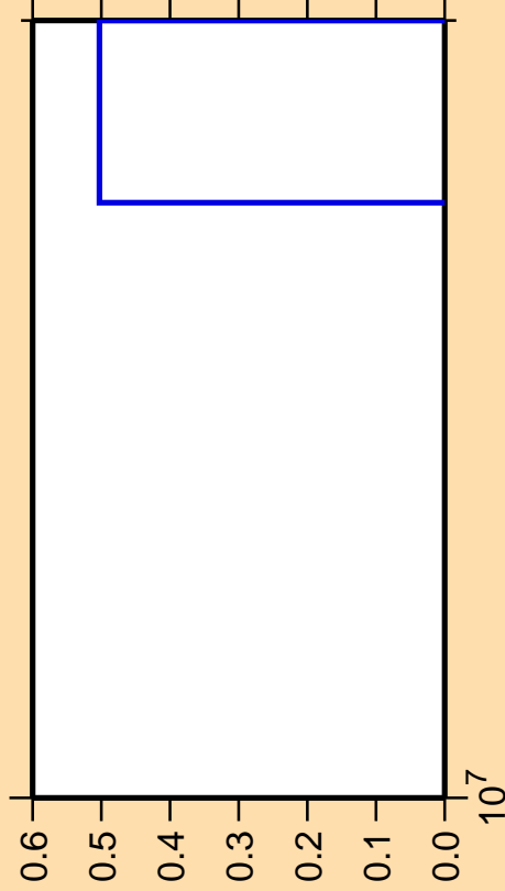
\Delta\sigma/\sigma vs. E for ^{108}\text{Pd}(n,2np)
