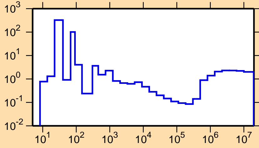
\sigma vs. E for ^{108}\text{Pd}(n,\text{nonel.})
