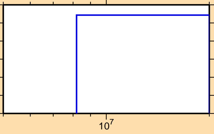
\sigma vs. E for ^{109}\text{Pd}(n,\text{nd})
