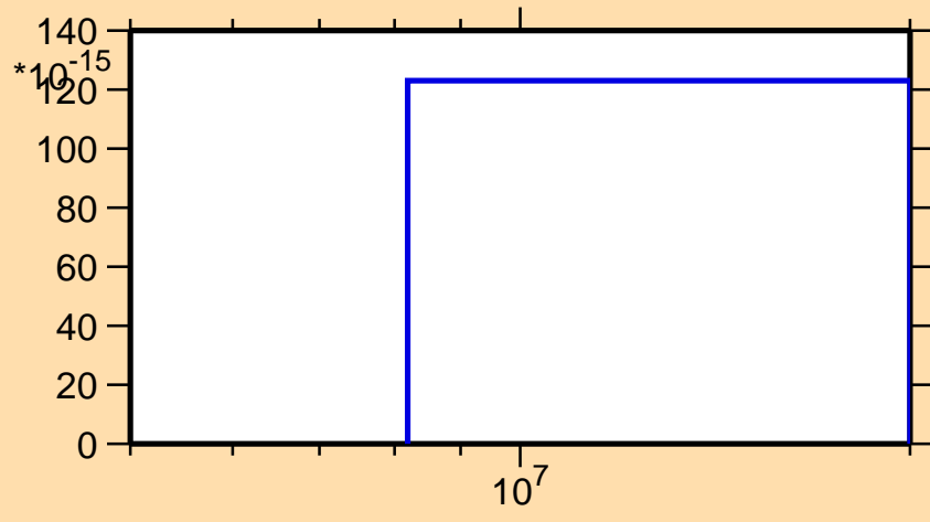
\sigma vs. E for ^{109}\text{Pd}(n,\text{He}3)
