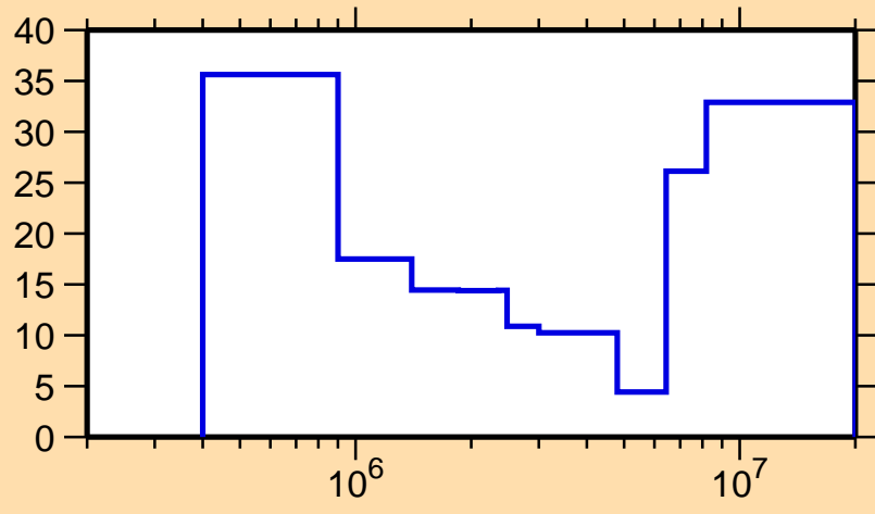
\Delta\sigma/\sigma vs. E for ^{109}\text{Pd}(n,n\text{cont.})
