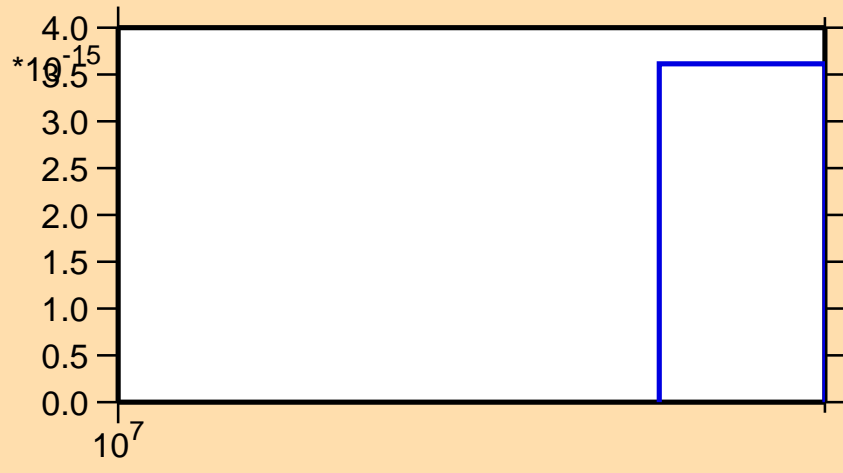
\sigma vs. E for ^{110}\text{Pd}(n,2np)
