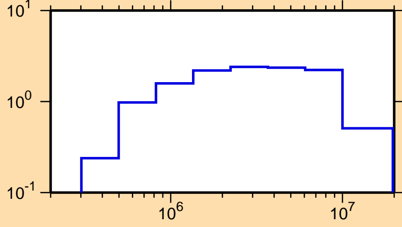
\sigma vs. E for ^{110}\text{Pd}(n,\text{inel.})
