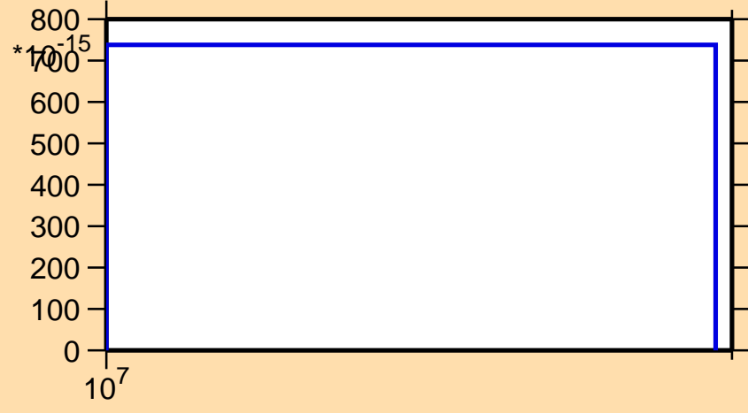
\sigma vs. E for ^{110}\text{Pd}(n,\text{nd})
