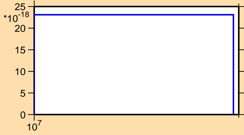
\sigma vs. E for ^{110}\text{Pd}(n,2np)
