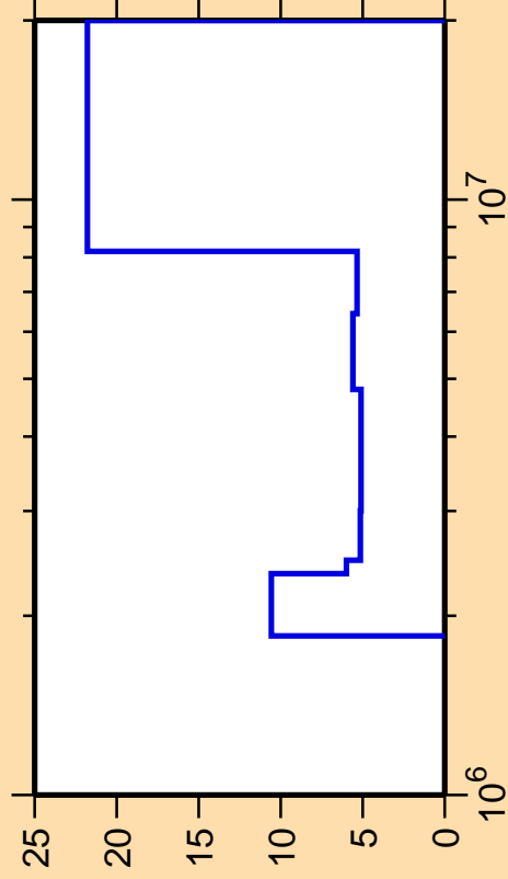
\Delta\sigma/\sigma vs. E for ^{110}\text{Pd}(n,n\text{cont.})
