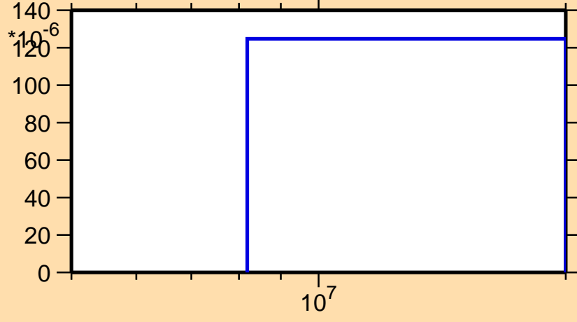
\sigma vs. E for ^{110}\text{Pd}(n,d)
