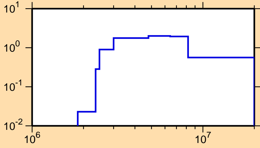
\sigma vs. E for ^{110}\text{Pd}(n,n\text{cont.})
