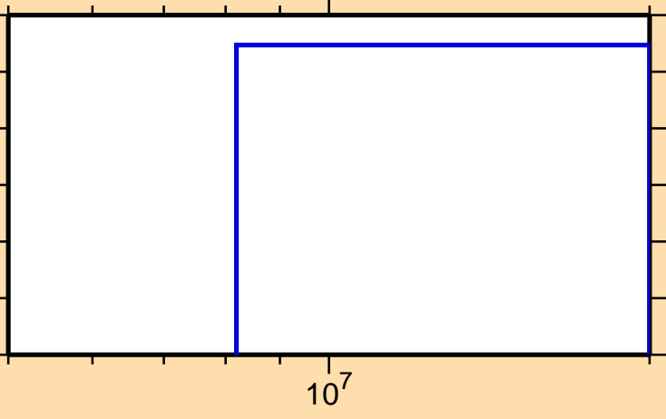
\sigma vs. E for ^{111}\text{Pd}(n,\text{nd})
