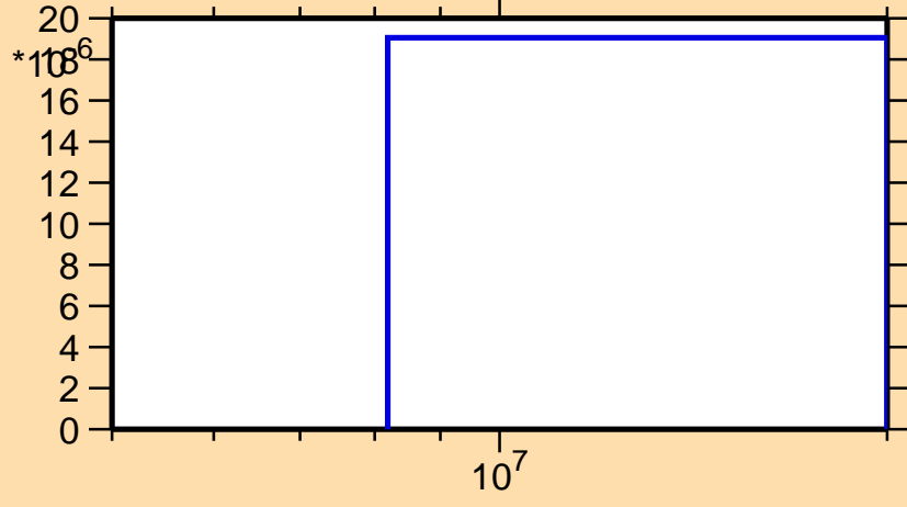
\sigma vs. E for ^{111}\text{Pd}(n,n\alpha)
