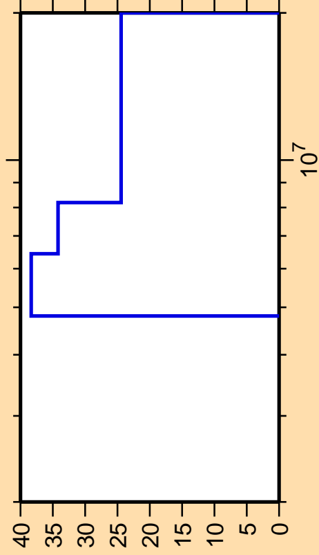
\Delta\sigma/\sigma vs. E for ^{111}\text{Pd}(n,2n)
