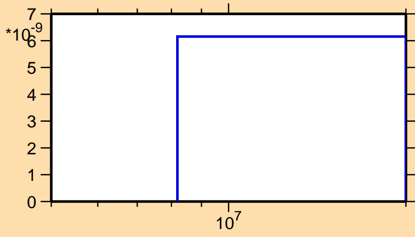
\sigma vs. E for ^{111}\text{Pd}(n,\text{nd})
