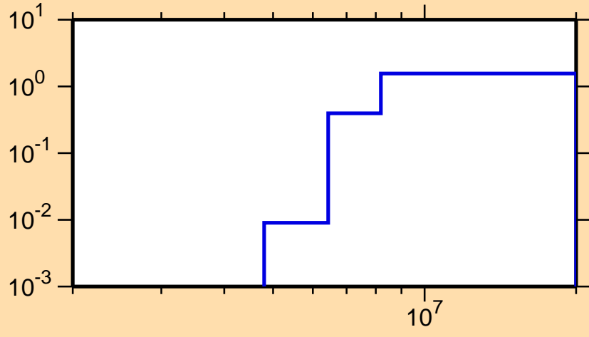
\sigma vs. E for ^{111}\text{Pd}(n,2n)
