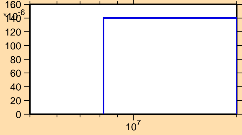
\sigma vs. E for ^{111}\text{Pd}(n,d)
