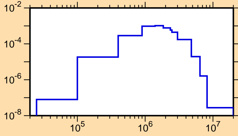
\sigma vs. E for ^{111}\text{Pd}(n,n_4)
