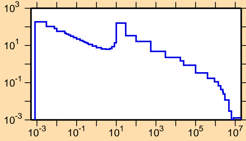
\sigma vs. E for ^{111}\text{Pd}(n,\gamma)
