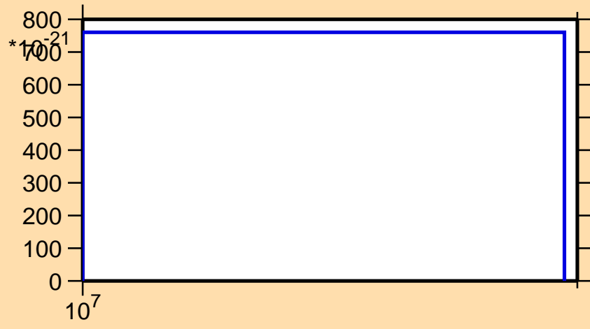
\sigma vs. E for ^{112}\text{Pd}(n,2np)
