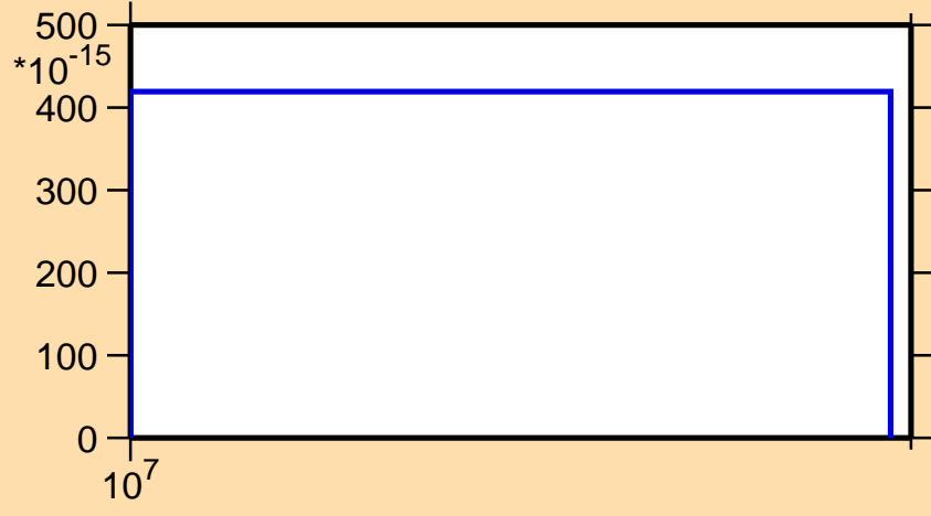
\sigma vs. E for ^{112}\text{Pd}(n,nt)
