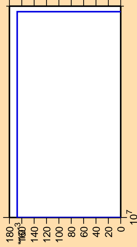
\Delta\sigma/\sigma vs. E for ^{112}\text{Pd}(n,nd)
