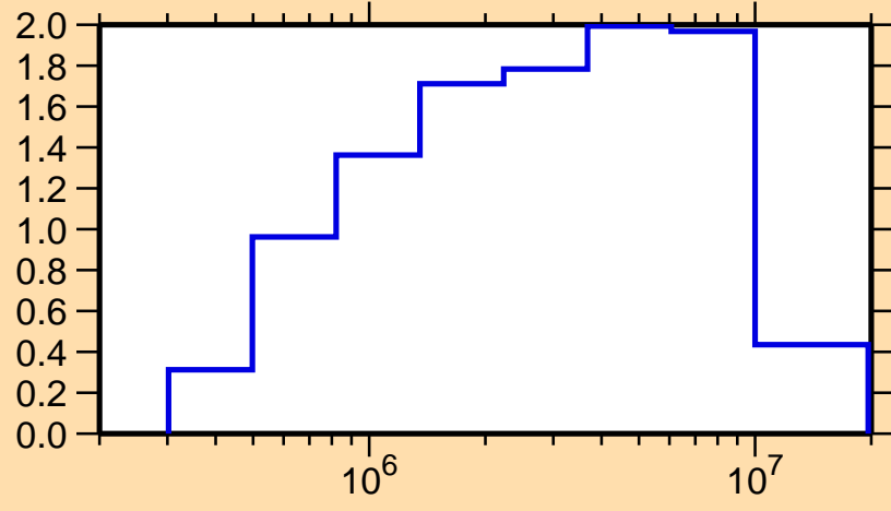
\sigma vs. E for ^{112}\text{Pd}(n,\text{inel.})
