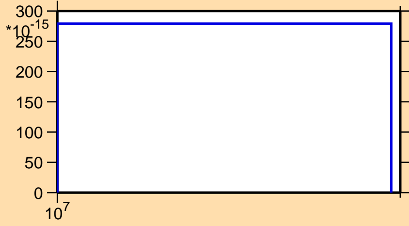
\sigma vs. E for ^{112}\text{Pd}(n,nd)
