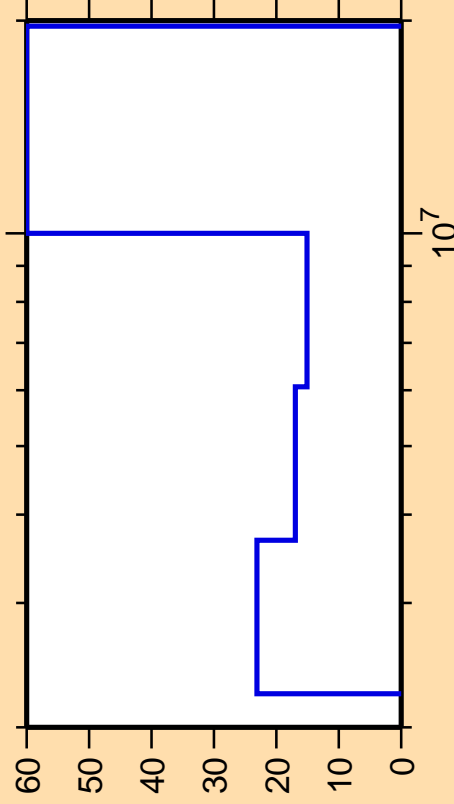
\Delta\sigma/\sigma vs. E for ^{112}\text{Pd}(n,n\text{cont.})
