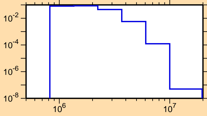
\sigma vs. E for ^{112}\text{Pd}(n,n_4)
