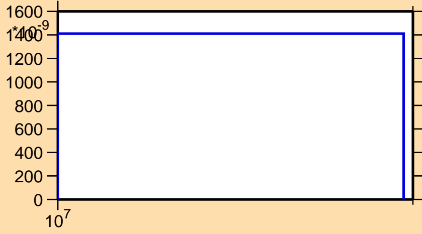
\sigma vs. E for ^{112}\text{Pd}(n,t)
