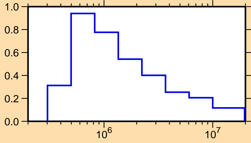
\sigma vs. E for ^{112}\text{Pd}(n,n_1)
