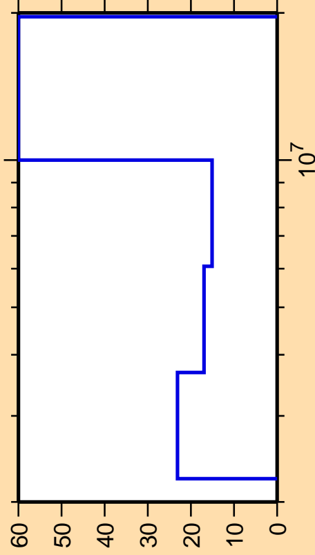
\Delta\sigma/\sigma vs. E for ^{112}\text{Pd}(n,n\text{cont.})
