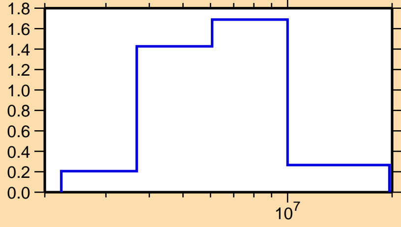
\sigma vs. E for ^{112}\text{Pd}(n,n\text{cont.})
