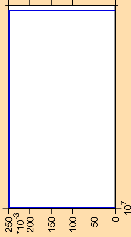
\Delta\sigma/\sigma vs. E for ^{112}\text{Pd}(n,2n\alpha)
