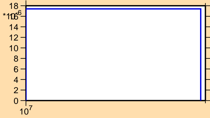
\sigma vs. E for ^{112}\text{Pd}(n,np)
