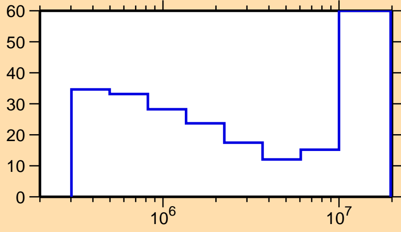
\Delta\sigma/\sigma vs. E for ^{112}\text{Pd}(n,\text{inel.})
