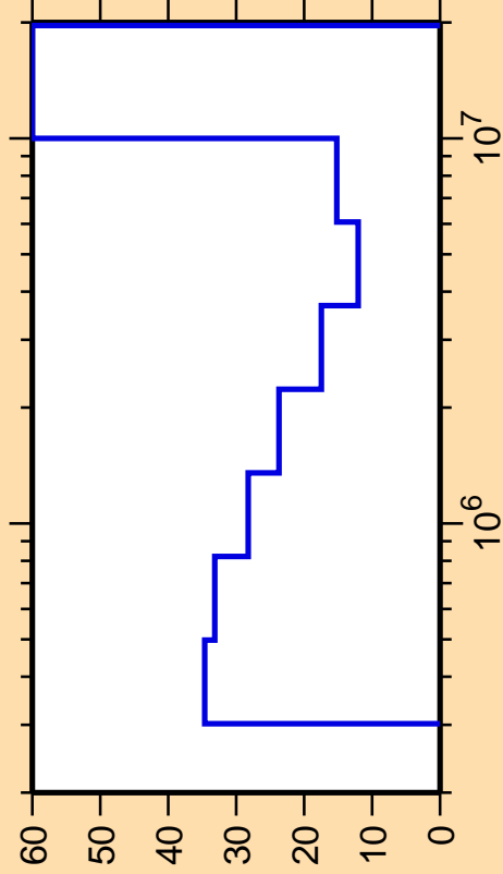
\Delta\sigma/\sigma vs. E for ^{112}\text{Pd}(n,\text{inel.})
