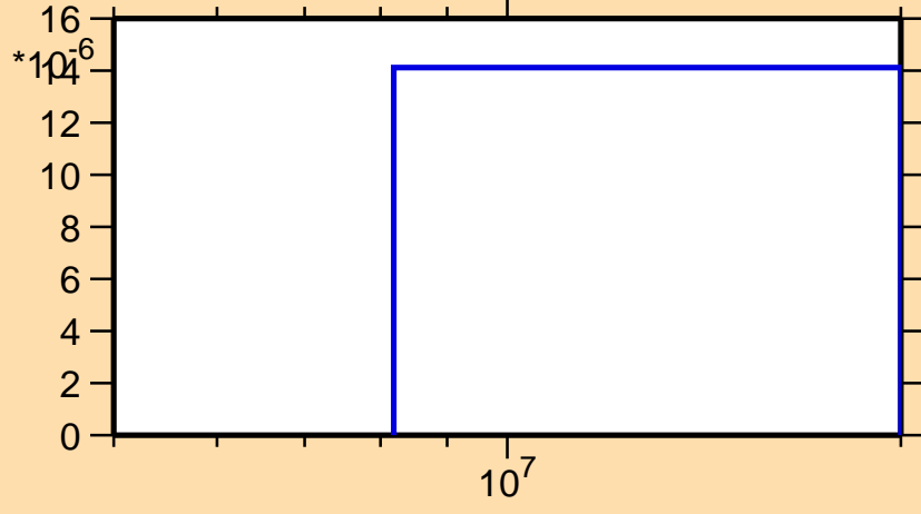
\sigma vs. E for ^{112}\text{Pd}(n,np)
