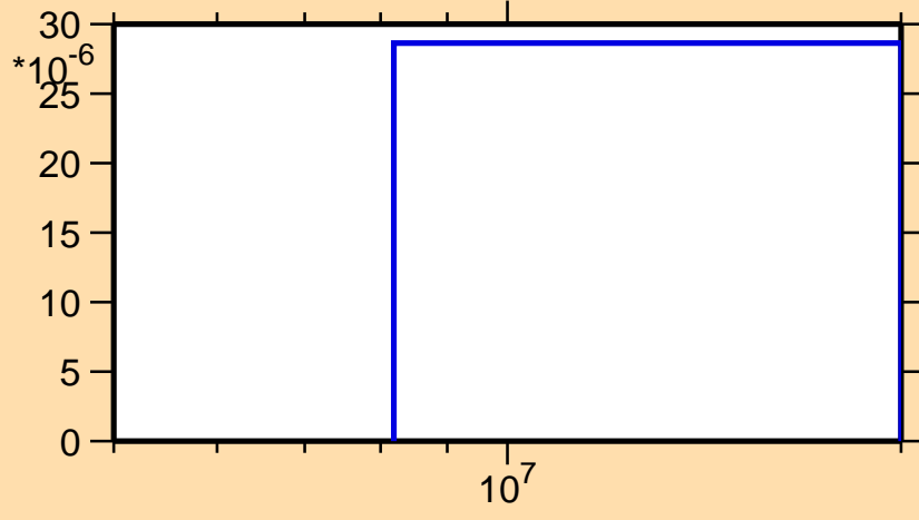
\sigma vs. E for ^{112}\text{Pd}(n,d)
