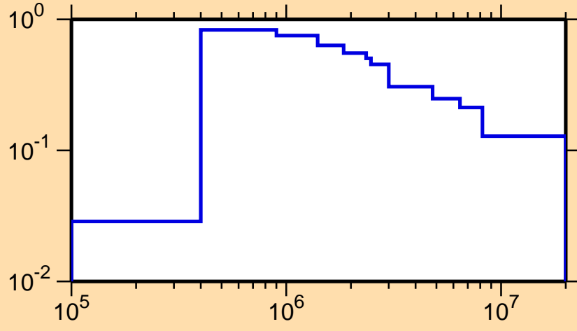
\sigma vs. E for ^{114}\text{Pd}(n,n_1)
