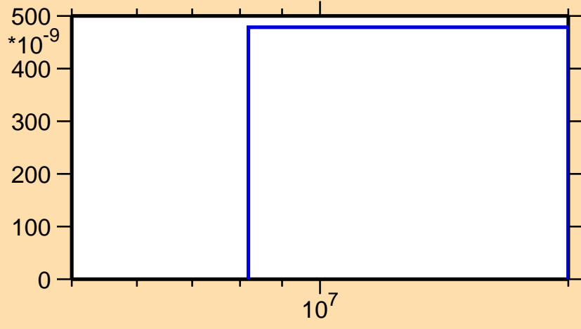
\sigma vs. E for ^{114}\text{Pd}(n,n\alpha)
