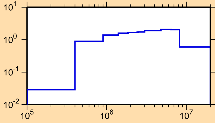
\sigma vs. E for ^{114}\text{Pd}(n,\text{inel.})
