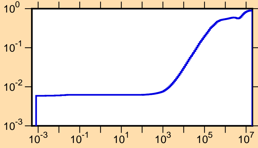
\mu vs. E for ^{115}\text{Pd}(\text{mt251})
