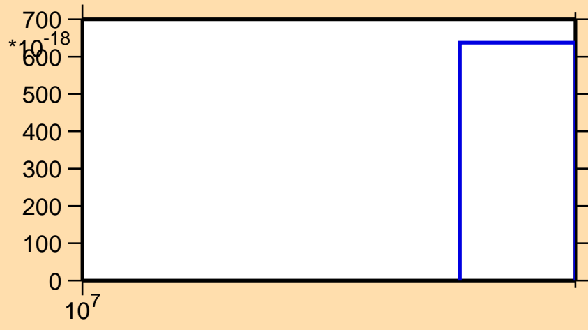
\sigma vs. E for ^{116}\text{Pd}(n,2np)
