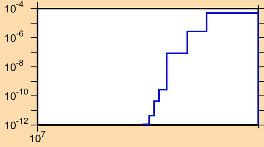
\sigma vs. E for ^{116}\text{Pd}(n,np)
