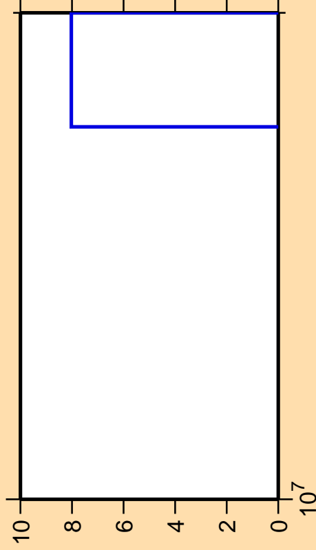
\Delta\sigma/\sigma vs. E for ^{116}\text{Pd}(n,\text{nd})
