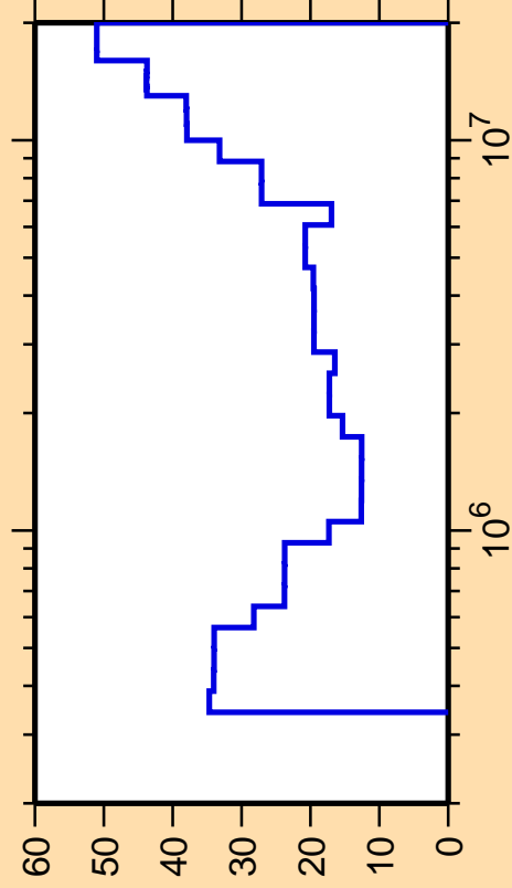
\Delta\sigma/\sigma vs. E for ^{116}\text{Pd}(n,\text{inel.})
