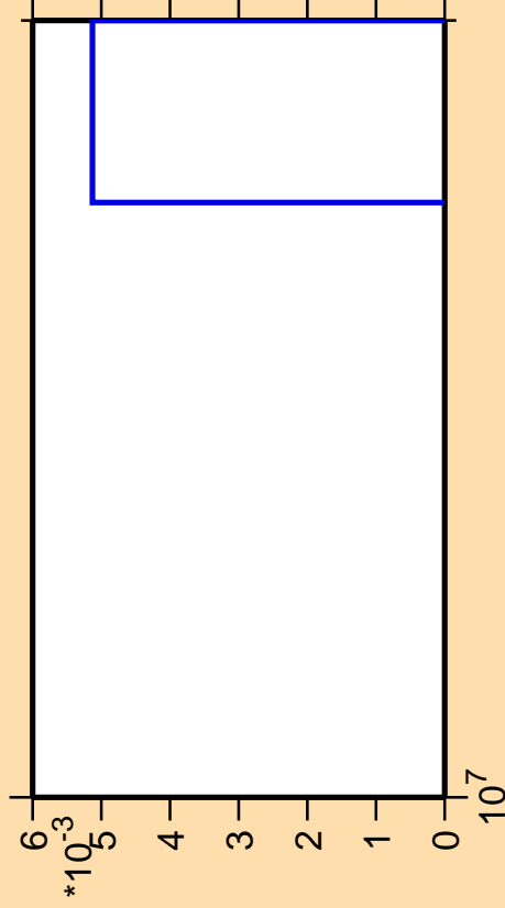
\Delta\sigma/\sigma vs. E for ^{116}\text{Pd}(n,2np)
