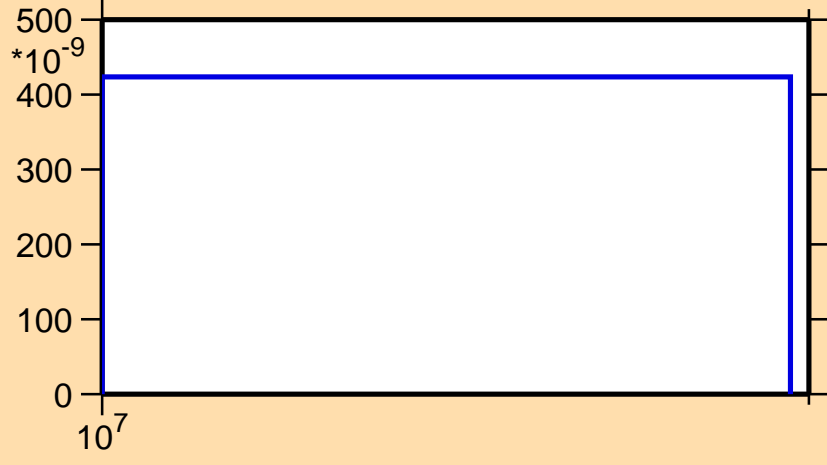
\sigma vs. E for ^{116}\text{Pd}(n,t)
