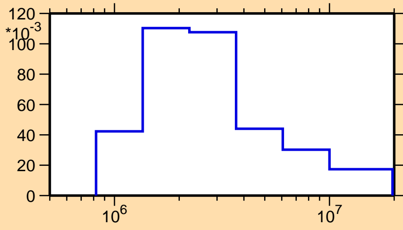
\sigma vs. E for ^{116}\text{Pd}(n,n_3)
