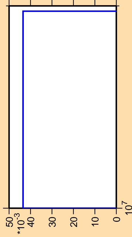
\Delta\sigma/\sigma vs. E for ^{116}\text{Pd}(n,\text{nd})
