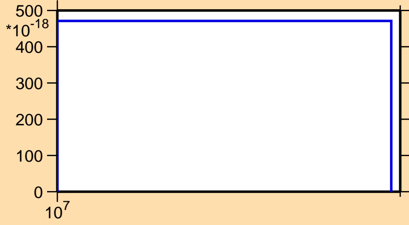
\sigma vs. E for ^{116}\text{Pd}(n,2n\alpha)
