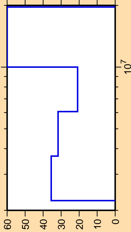
\Delta\sigma/\sigma vs. E for ^{116}\text{Pd}(n,n\text{cont.})
