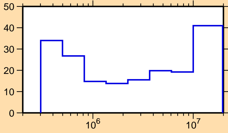
\Delta\sigma/\sigma vs. E for ^{116}\text{Pd}(n,\text{inel.})
