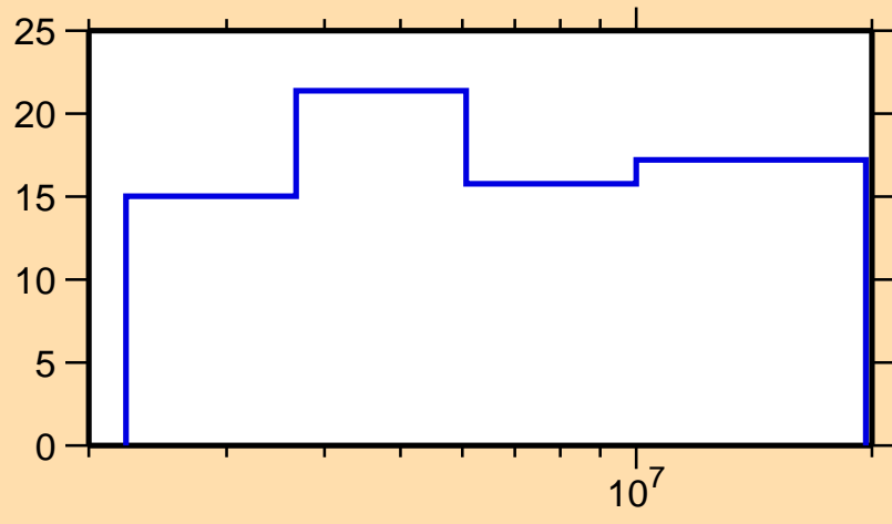
\Delta\sigma/\sigma vs. E for ^{116}\text{Pd}(n,\text{tot.})
