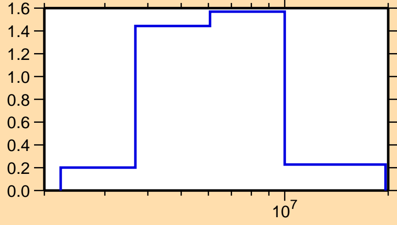
\sigma vs. E for ^{116}\text{Pd}(n,n\text{cont.})
