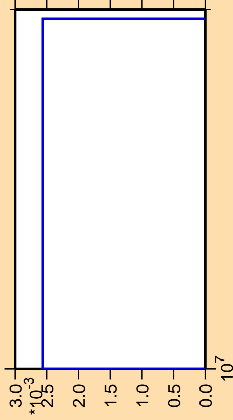
\Delta\sigma/\sigma vs. E for ^{116}\text{Pd}(n,2n\alpha)
