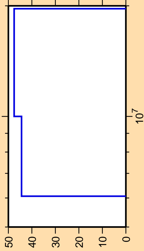
\Delta\sigma/\sigma vs. E for ^{116}\text{Pd}(n,2n)
