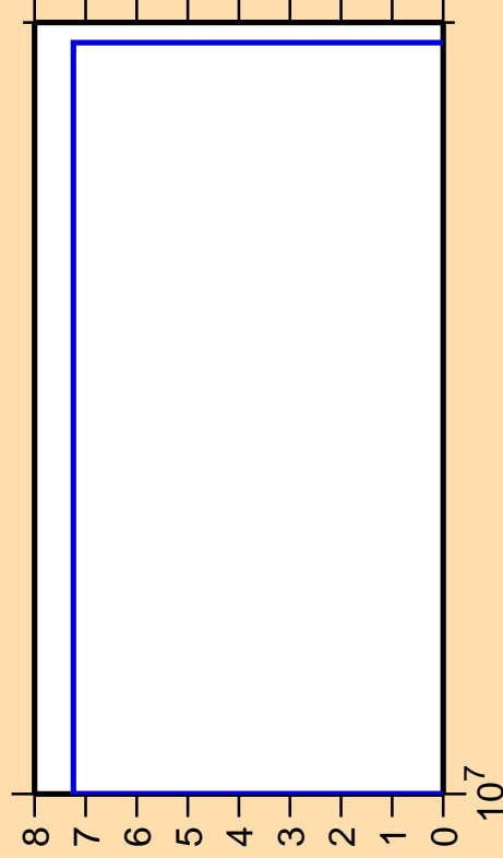
\Delta\sigma/\sigma vs. E for ^{116}\text{Pd}(n,nt)
