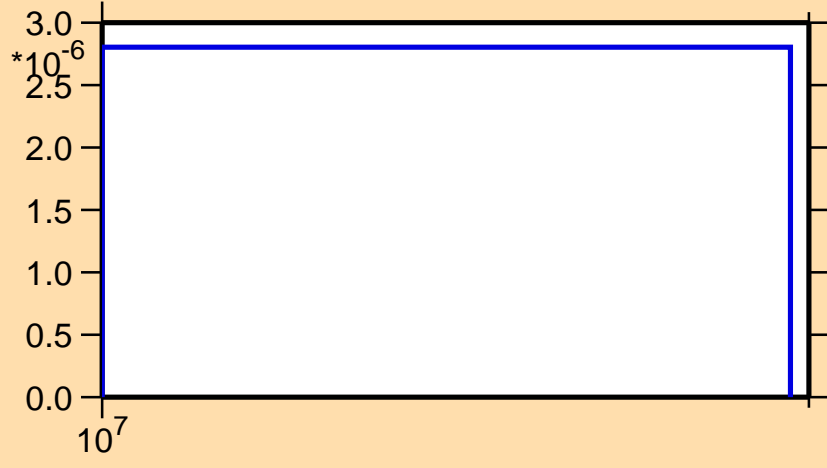
\sigma vs. E for ^{116}\text{Pd}(n,d)
