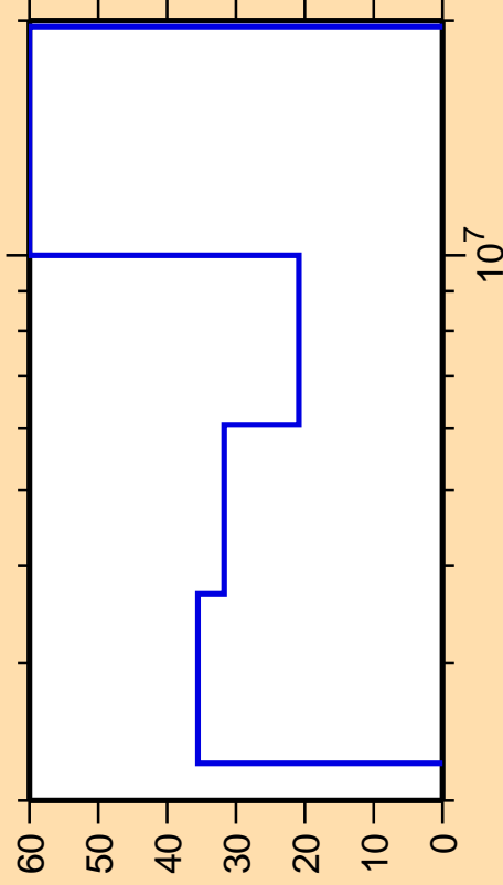
\Delta\sigma/\sigma vs. E for ^{116}\text{Pd}(n,n\text{cont.})
