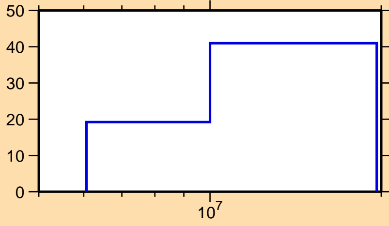
\Delta\sigma/\sigma vs. E for ^{116}\text{Pd}(n,\text{inel.})
