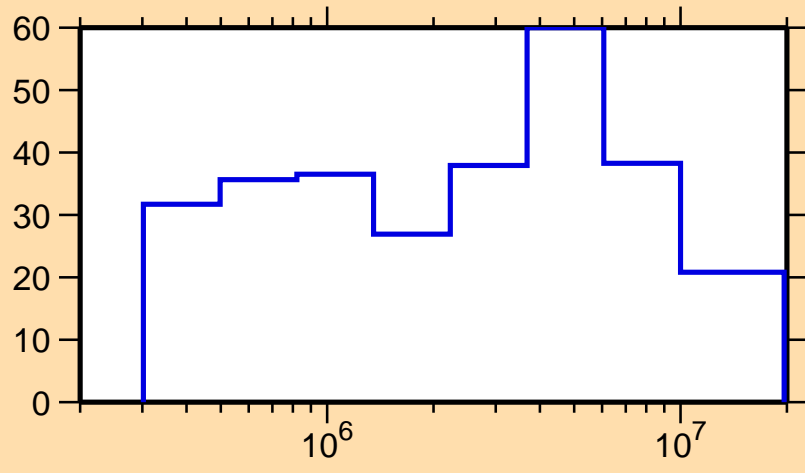
\Delta\sigma/\sigma vs. E for ^{116}\text{Pd}(n,\text{el.})
