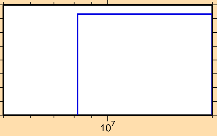
\sigma vs. E for ^{116}\text{Pd}(n,\text{nd})
