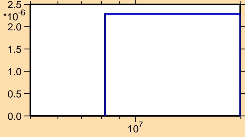
\sigma vs. E for ^{116}\text{Pd}(n,d)
