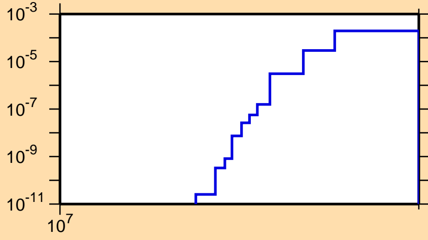
\sigma vs. E for ^{117}\text{Pd}(n,d)
