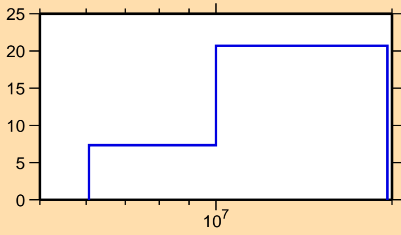
\Delta\sigma/\sigma vs. E for ^{117}\text{Pd}(n,\text{el.})
