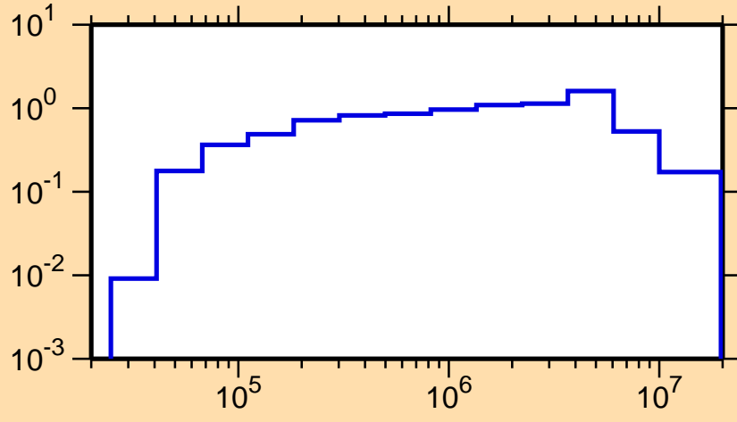
\sigma vs. E for ^{117}\text{Pd}(n,\text{inel.})
