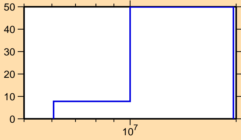
\Delta\sigma/\sigma vs. E for ^{117}\text{Pd}(n,2n)
