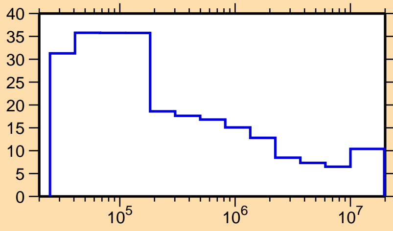
\Delta\sigma/\sigma vs. E for ^{117}\text{Pd}(n,\text{nonel.})
