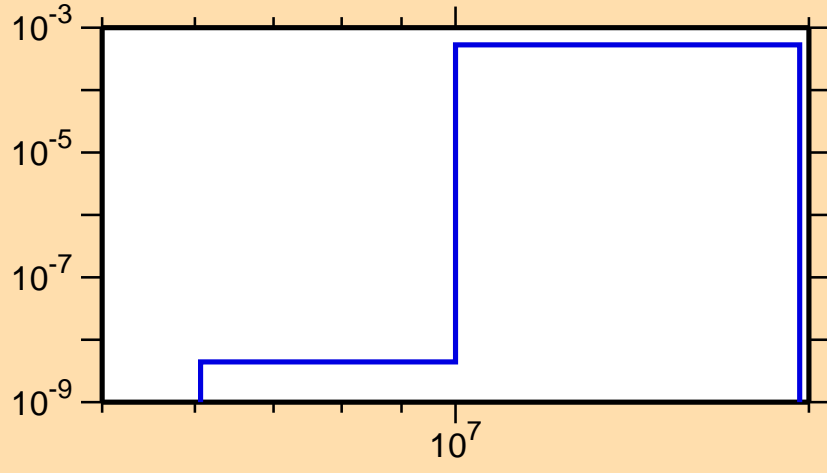
\sigma vs. E for ^{117}\text{Pd}(n,p)
