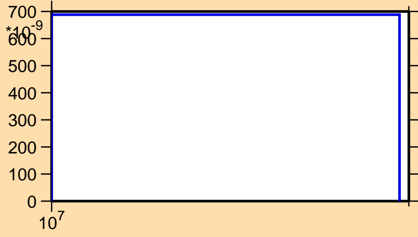
\sigma vs. E for ^{117}\text{Pd}(n,np)
