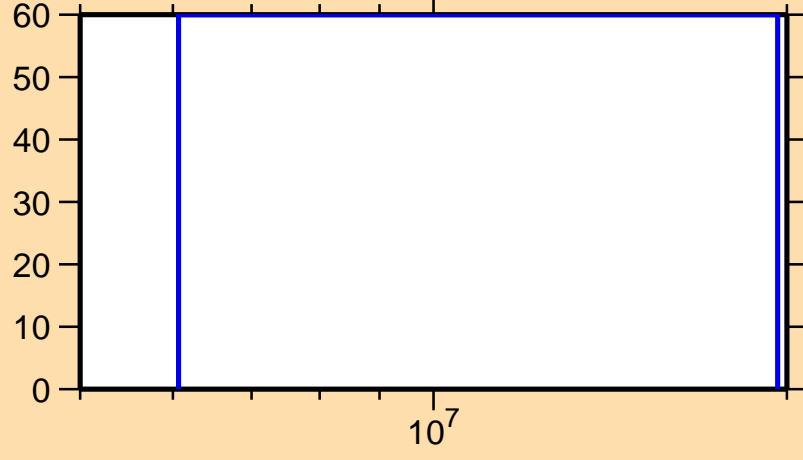
\Delta\sigma/\sigma vs. E for ^{117}\text{Pd}(n,\gamma)
