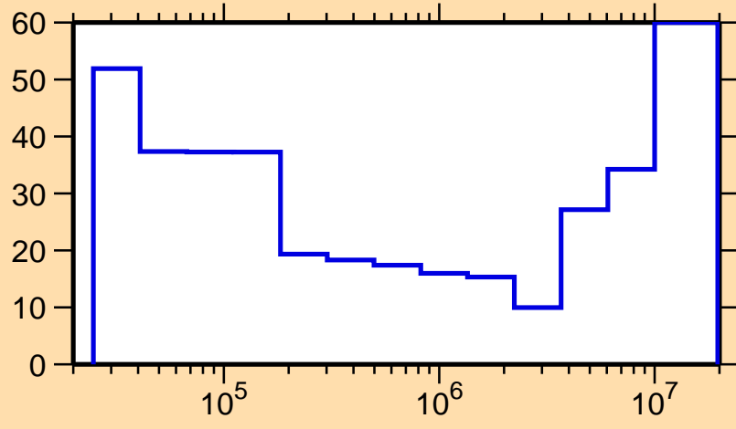
\Delta\sigma/\sigma vs. E for ^{117}\text{Pd}(n,\text{inel.})
