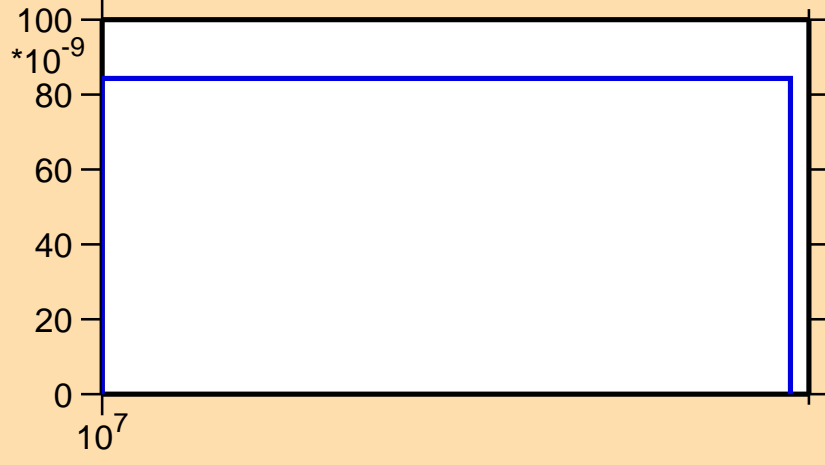
\sigma vs. E for ^{117}\text{Pd}(n,n\alpha)
