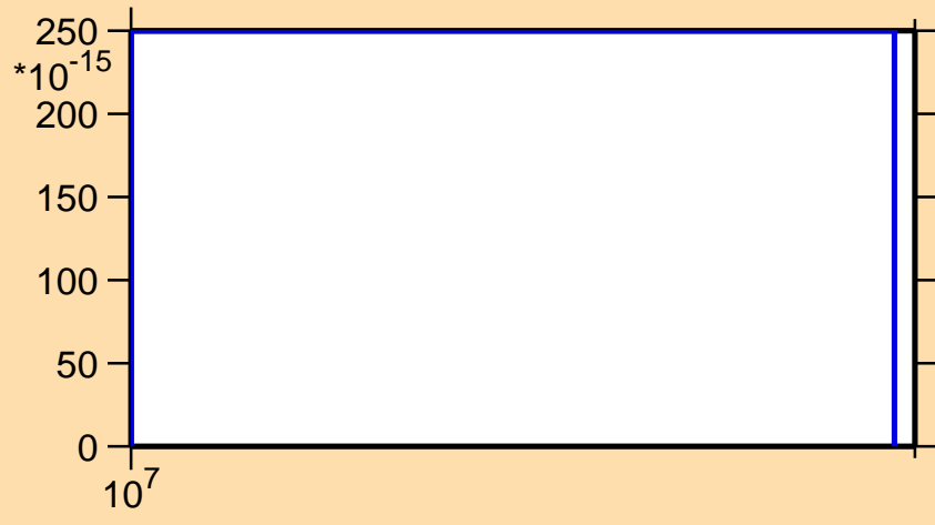
\sigma vs. E for ^{117}\text{Pd}(n,2np)
