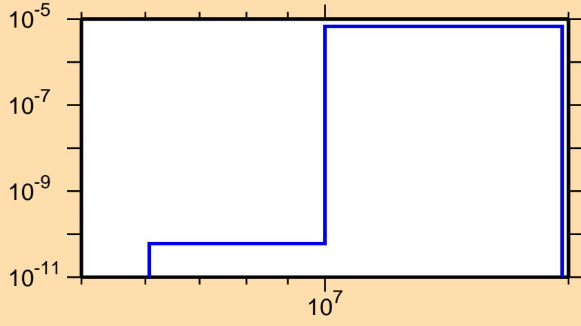
\sigma vs. E for ^{117}\text{Pd}(n,\alpha)
