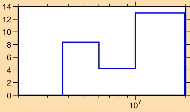
\Delta\sigma/\sigma vs. E for ^{117}\text{Pd}(n,\text{tot.})
