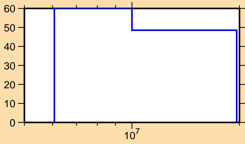
\Delta\sigma/\sigma vs. E for ^{117}\text{Pd}(n,n\text{cont.})
