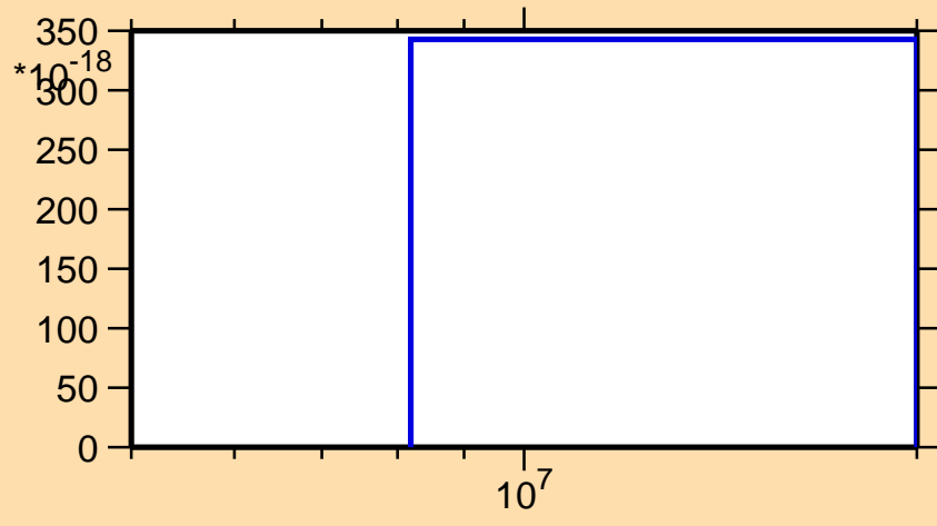
\sigma vs. E for ^{118}\text{Pd}(n,nd)
