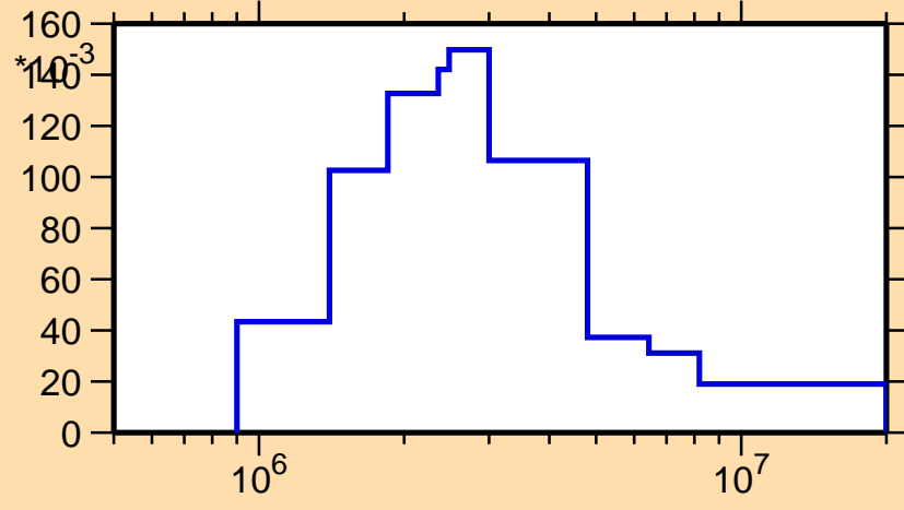
\sigma vs. E for ^{118}\text{Pd}(n,n_3)
