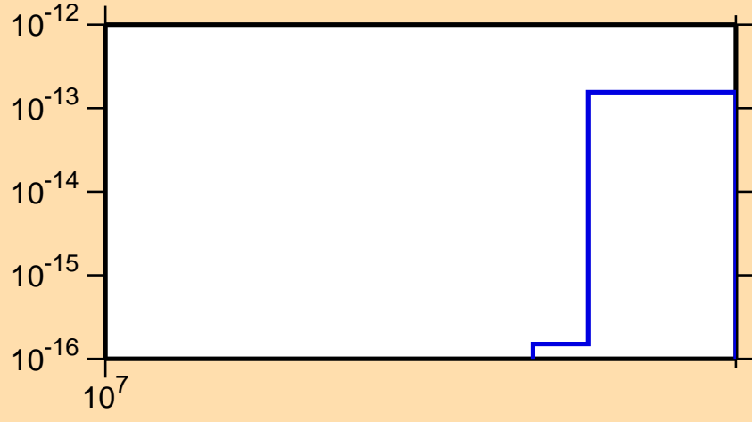
\sigma vs. E for ^{127}\text{Pm}(n,2n\alpha)
