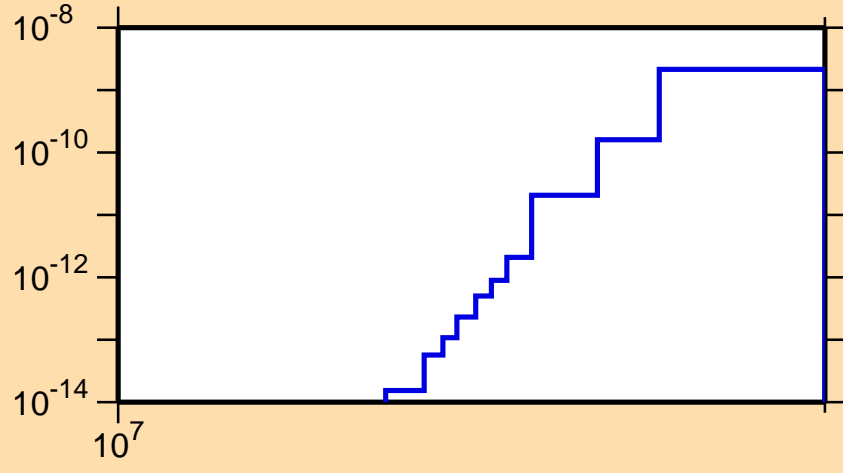
\sigma vs. E for ^{127}\text{Pm} (mt 34)
