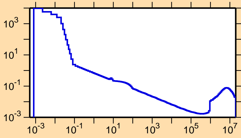
\sigma vs. E for ^{127}\text{Pm}(n,\alpha)
