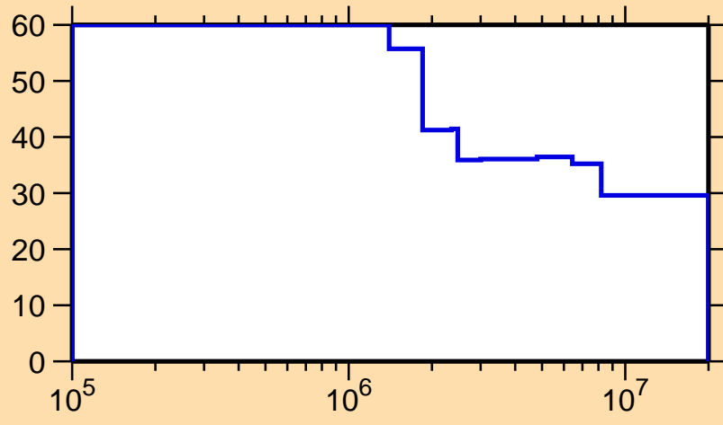
\Delta\sigma/\sigma vs. E for ^{127}\text{Pm}(n,n_1)
