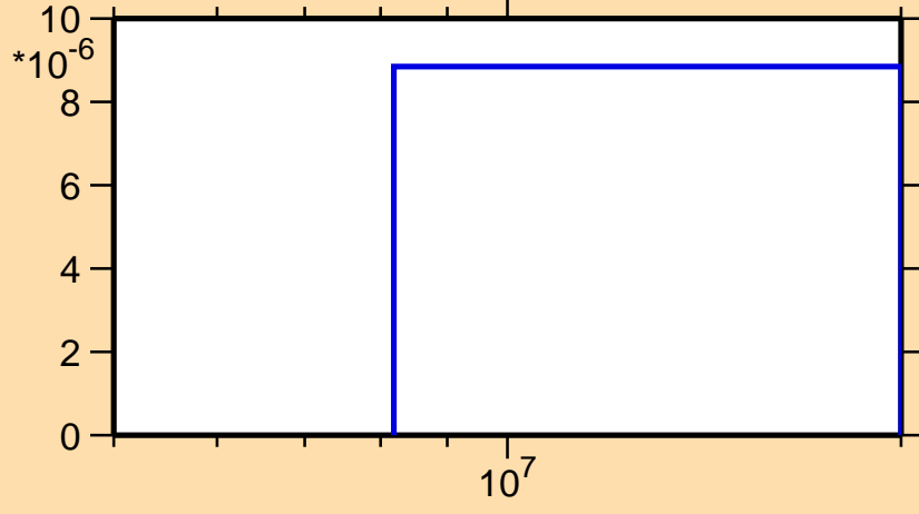
\sigma vs. E for ^{127}\text{Pm}(n,pt)
