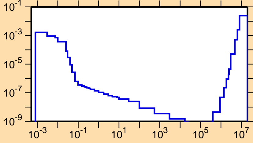
\sigma vs. E for ^{127}\text{Pm}(n,d)
