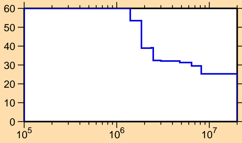
\Delta\sigma/\sigma vs. E for ^{127}\text{Pm}(n,\text{inel.})
