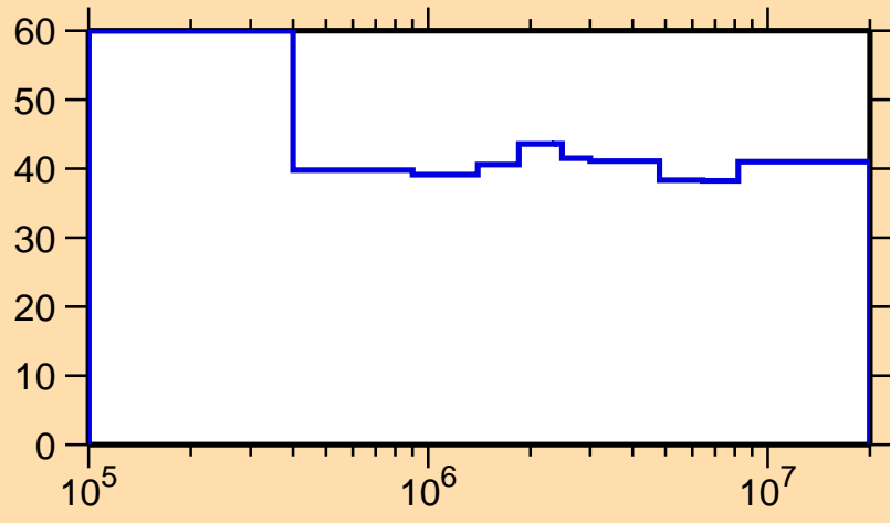
\Delta\sigma/\sigma vs. E for ^{127}\text{Pm}(n,ncont.)
