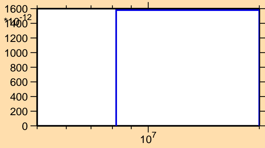
\sigma vs. E for ^{127}\text{Pm}(n,nd)
