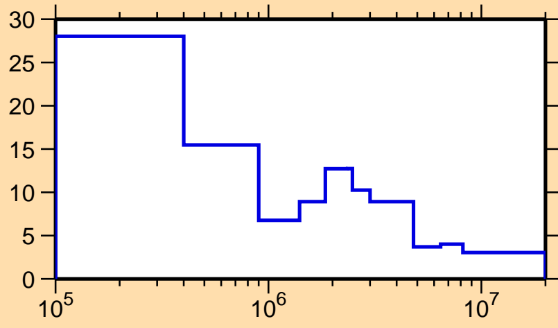
\Delta\sigma/\sigma vs. E for ^{127}\text{Pm}(n,\text{tot.})
