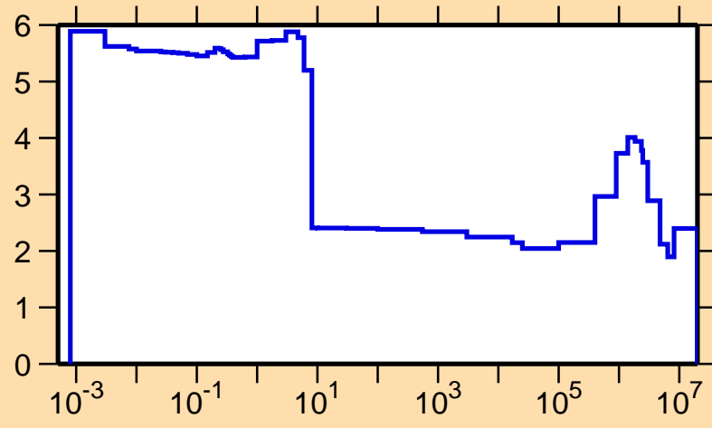
\sigma vs. E for ^{127}\text{Pm}(n,\text{el.})
