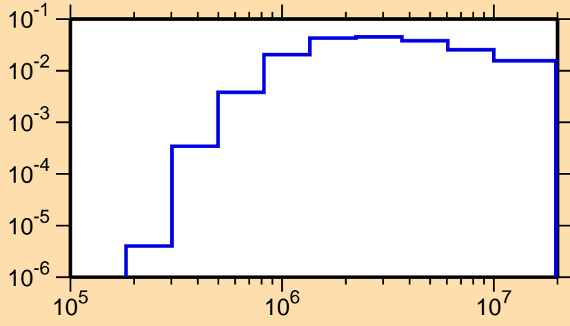
\sigma vs. E for ^{128}\text{Pm}(n,n_1)
