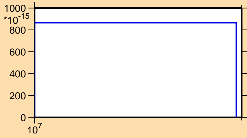
\sigma vs. E for ^{128}\text{Pm}(n,2n\alpha)
