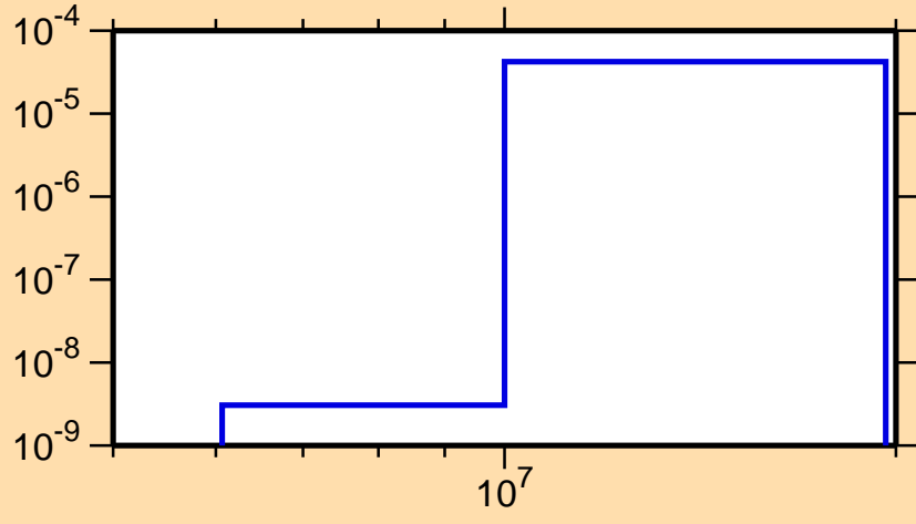
\sigma vs. E for ^{128}\text{Pm} (mt 45)
