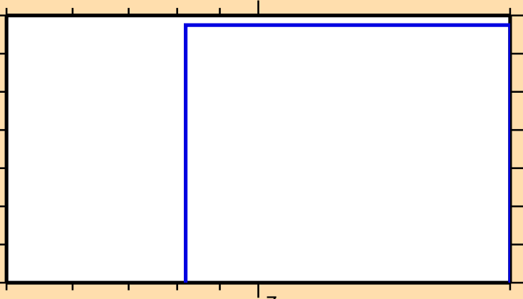
\sigma vs. E for ^{128}\text{Pm}(n,2np)
