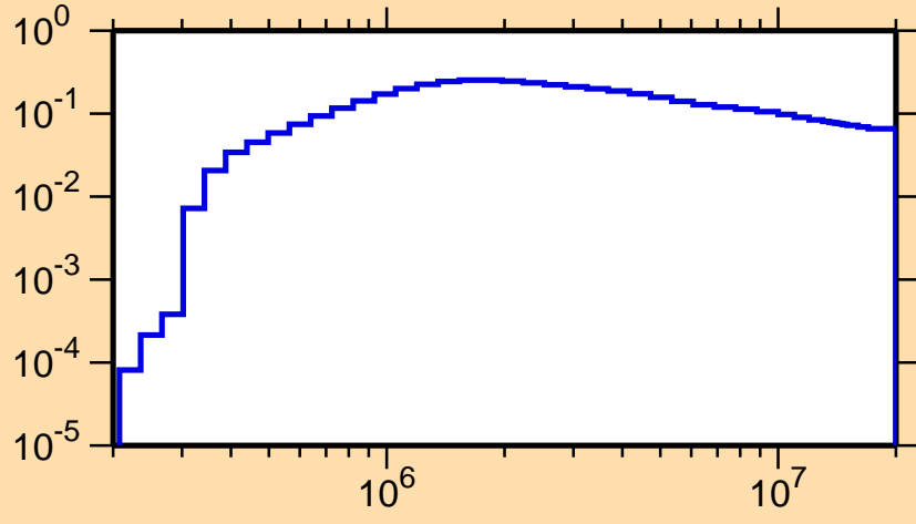
\sigma vs. E for ^{129}\text{Pm}(n,\text{inel.})
