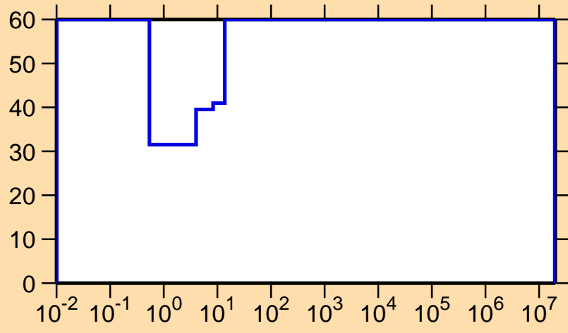
\Delta\sigma/\sigma vs. E for ^{129}\text{Pm}(n,\gamma)
