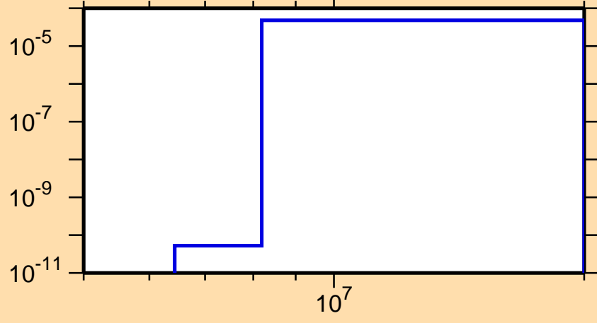
\sigma vs. E for ^{129}\text{Pm} (mt 45)
