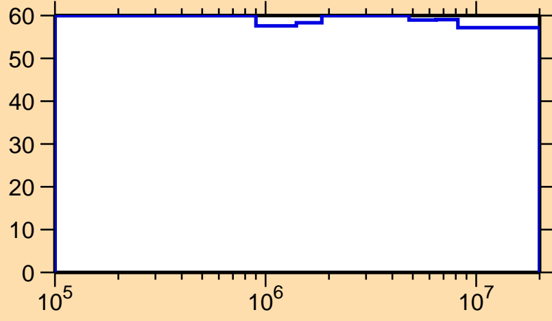
\Delta\sigma/\sigma vs. E for ^{129}\text{Pm}(n,n\text{cont.})
