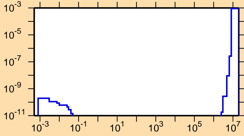
\sigma vs. E for ^{129}\text{Pm}(n,\text{He}3)
