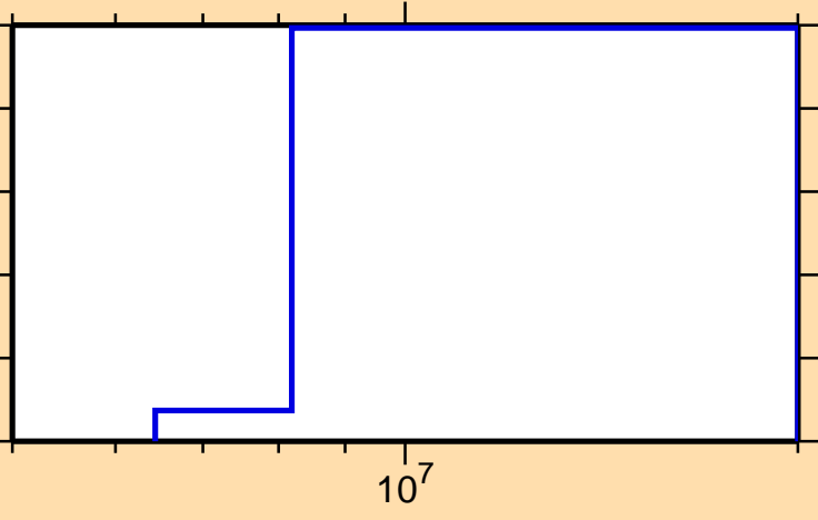
\sigma vs. E for ^{129}\text{Pm}(\text{mt117})
