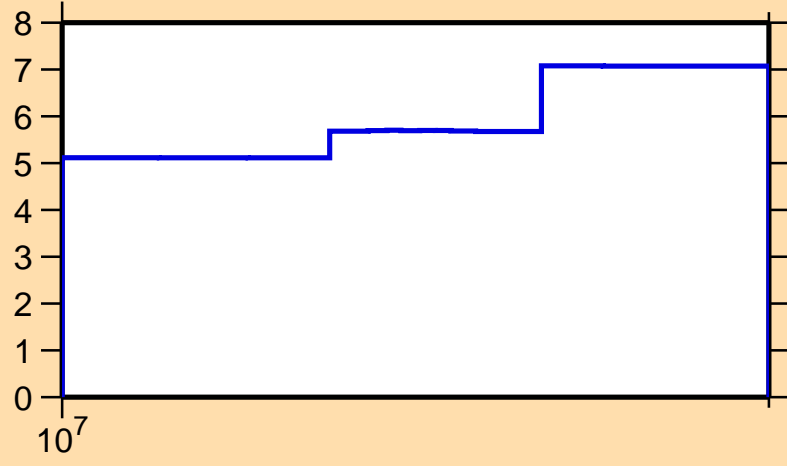
\Delta\sigma/\sigma vs. E for ^{130}\text{Pm}(n,el.)
