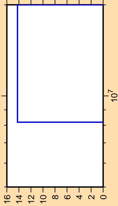
\Delta\sigma/\sigma vs. E for ^{130}\text{Pm}(n,p)
