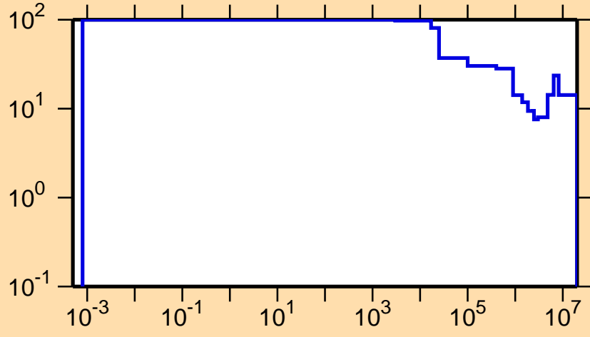
\Delta\sigma/\sigma vs. E for ^{130}\text{Pm}(n,p)
