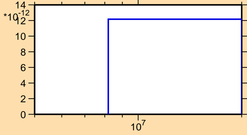
\sigma vs. E for ^{130}\text{Pm}(n,2n\alpha)
