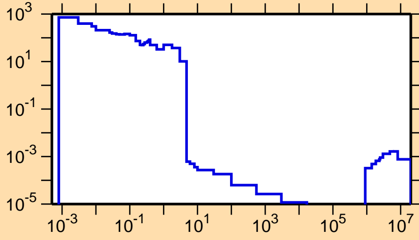
\sigma vs. E for ^{130}\text{Pm}(n,\gamma)
