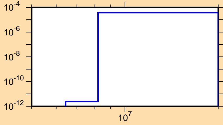
\sigma vs. E for ^{130}\text{Pm} (mt 45)
