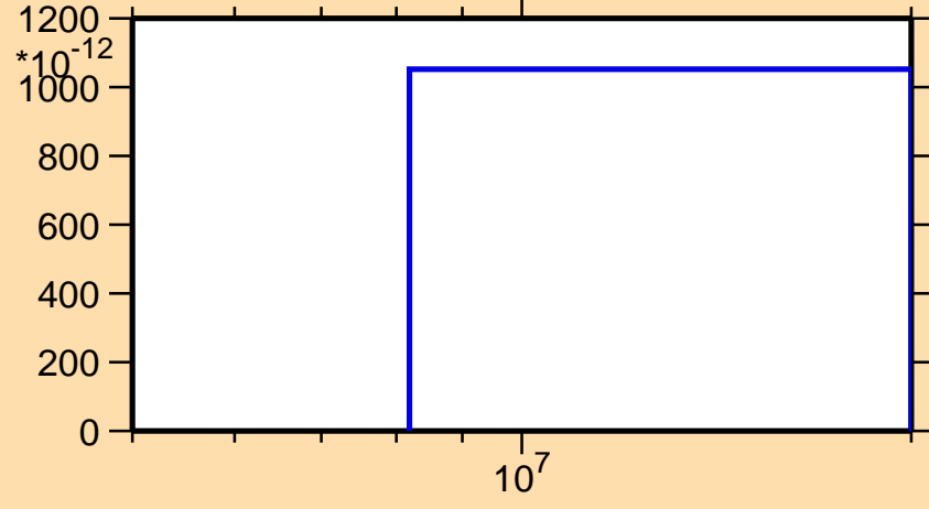
\sigma vs. E for ^{130}\text{Pm} (mt 34)
