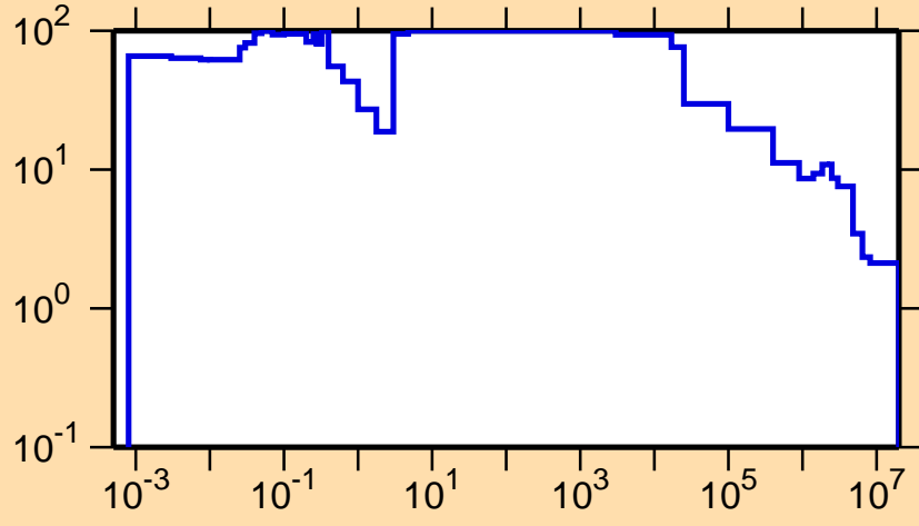
\Delta\sigma/\sigma vs. E for ^{130}\text{Pm}(n,\text{tot.})
