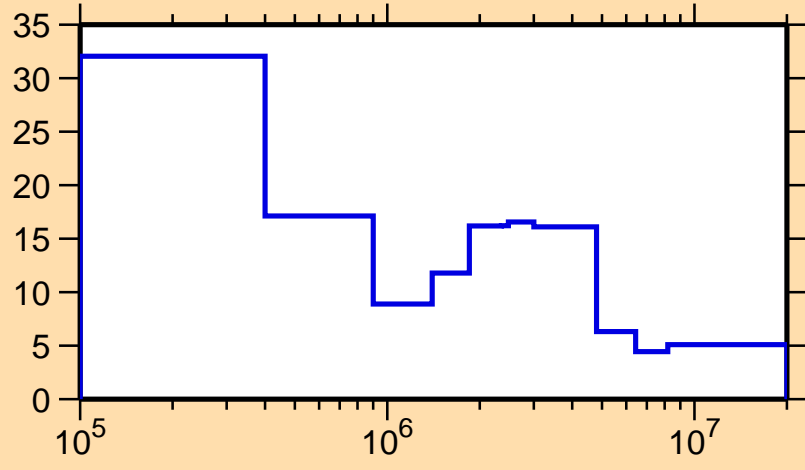
\Delta\sigma/\sigma vs. E for ^{130}\text{Pm}(n,\text{el.})
