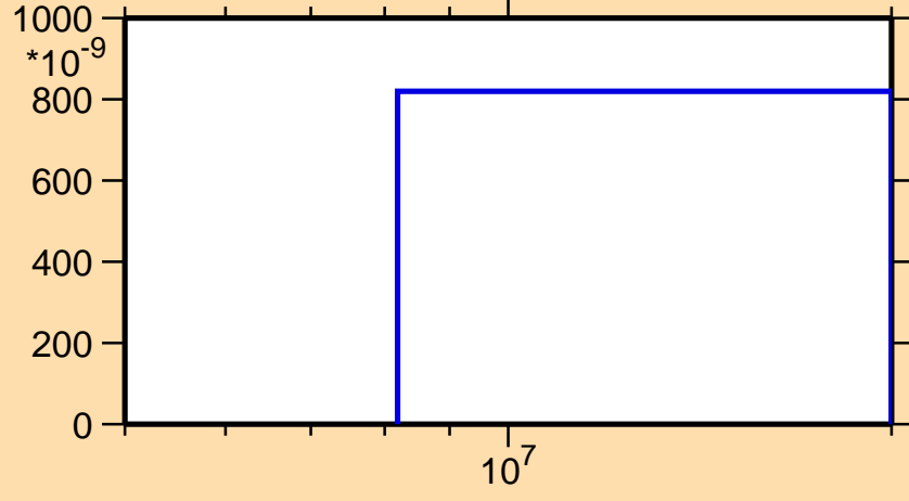
\sigma vs. E for ^{130}\text{Pm}(n,nd)
