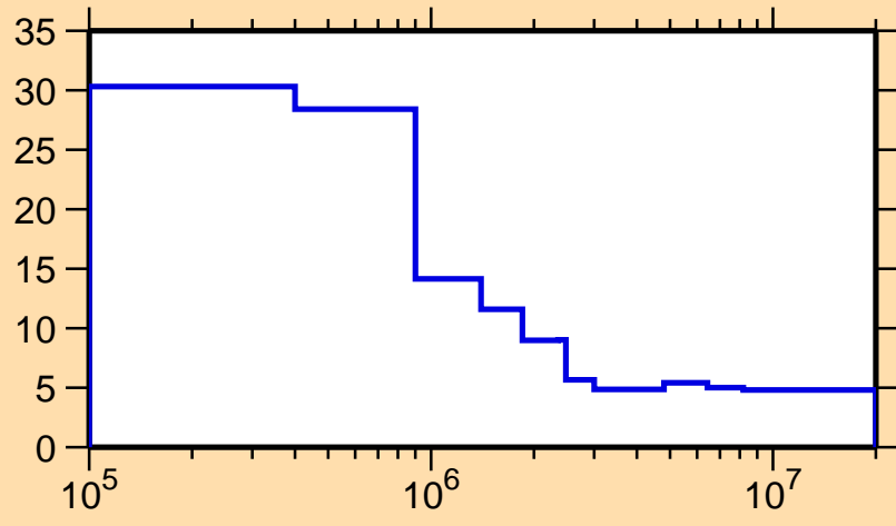
\Delta\sigma/\sigma vs. E for ^{130}\text{Pm}(n,\text{nonel.})
