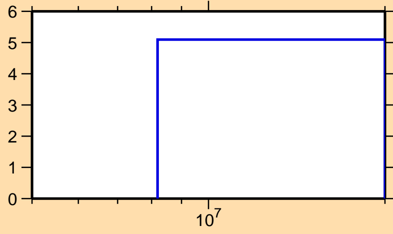
\Delta\sigma/\sigma vs. E for ^{130}\text{Pm}(n,\text{el.})
