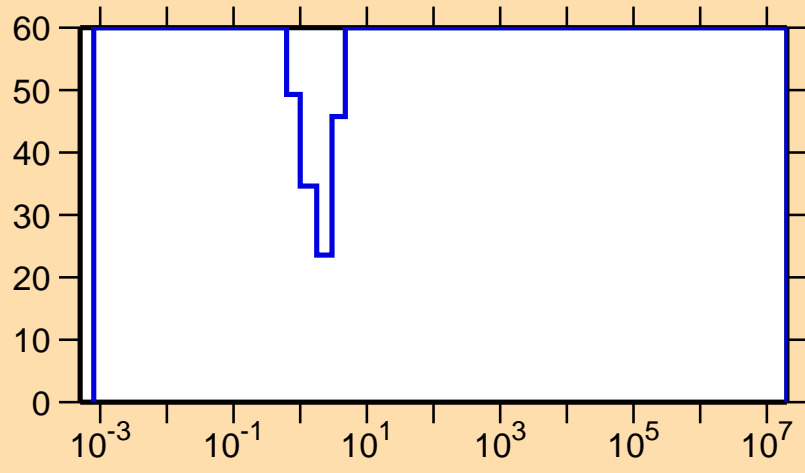
\Delta\sigma/\sigma vs. E for ^{130}\text{Pm}(n,\gamma)
