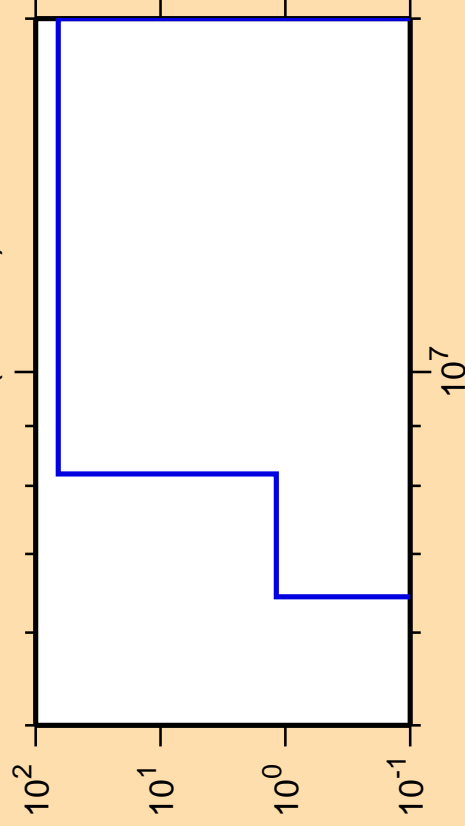
\Delta\sigma/\sigma vs. E for ^{130}\text{Pm}(\text{mt117})
