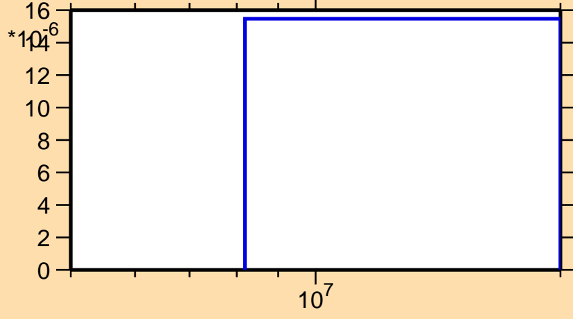
\sigma vs. E for ^{130}\text{Pm}(n,pt)
