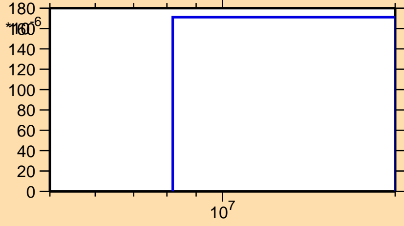
\sigma vs. E for ^{130}\text{Pm}(n,2n)
