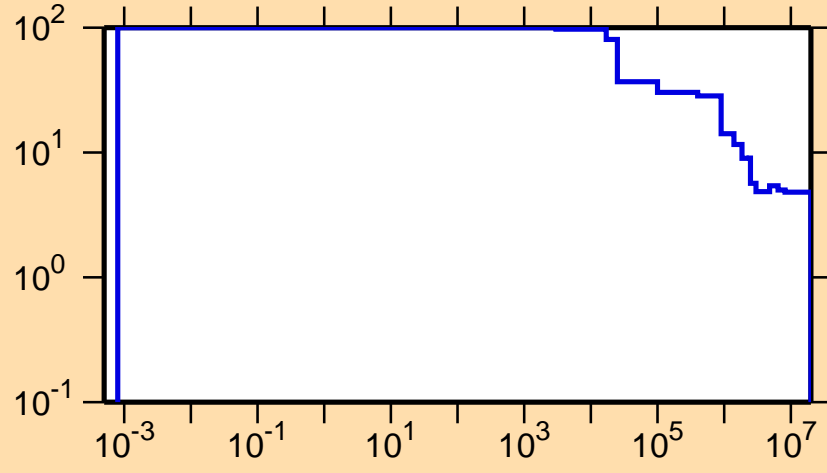
\Delta\sigma/\sigma vs. E for ^{130}\text{Pm}(n,\text{nonel.})
