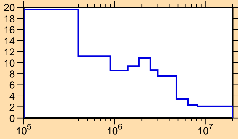
\Delta\sigma/\sigma vs. E for ^{130}\text{Pm}(n, \text{tot.})
