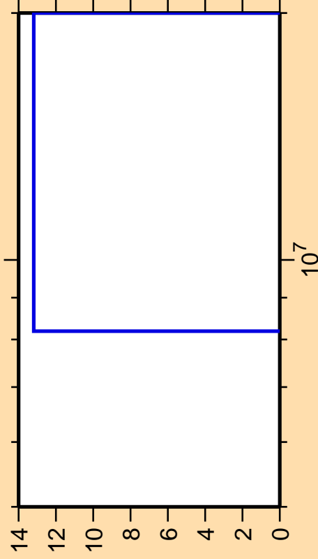
\Delta\sigma/\sigma vs. E for ^{130}\text{Pm}(n,n\text{cont.})
