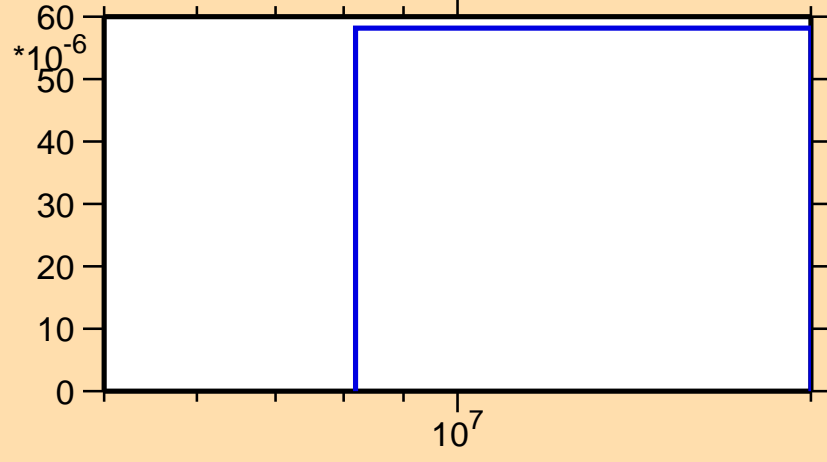
\sigma vs. E for ^{130}\text{Pm}(n,2np)
