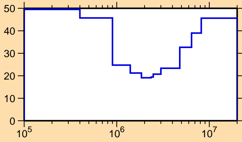
\Delta\sigma/\sigma vs. E for ^{130}\text{Pm}(n,n_1)
