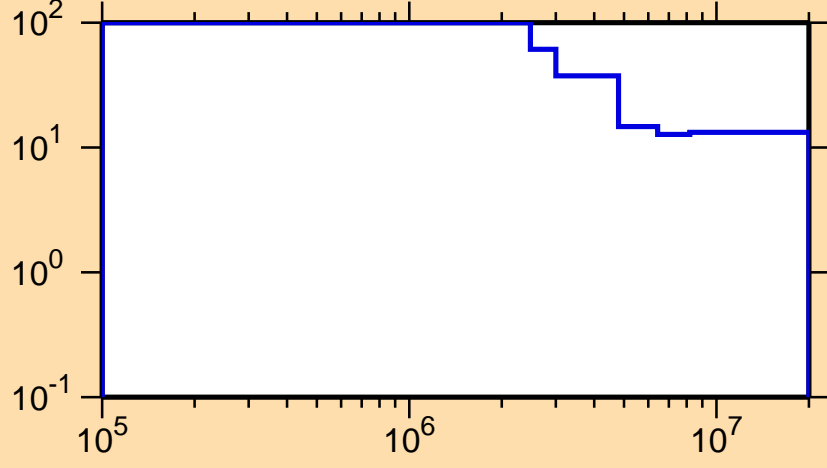
\Delta\sigma/\sigma vs. E for ^{130}\text{Pm}(n,\text{inel.})
