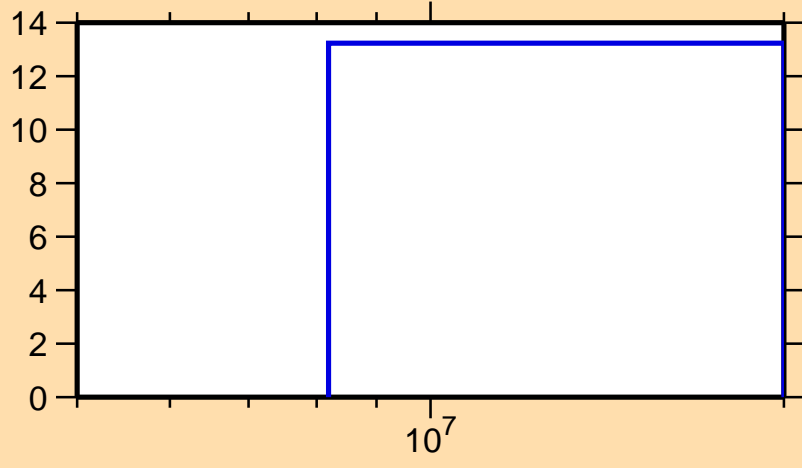
\Delta\sigma/\sigma vs. E for ^{130}\text{Pm}(n,\text{inel.})
