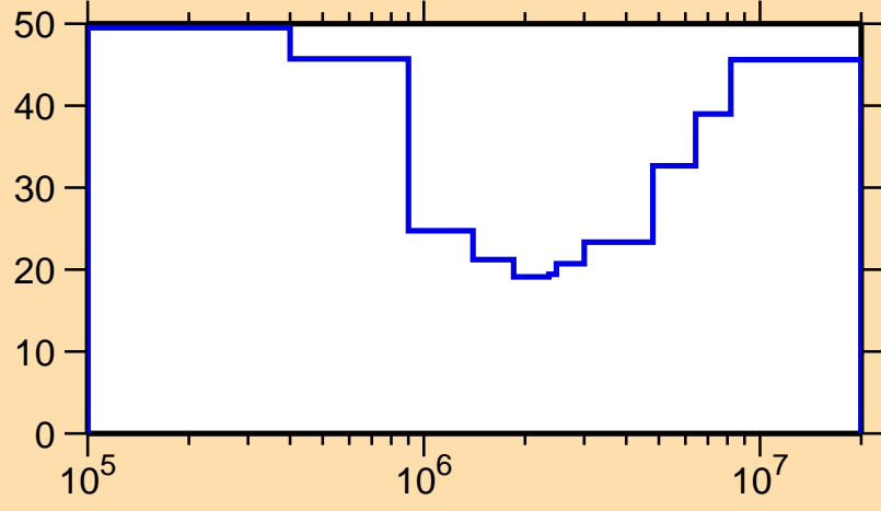
\Delta\sigma/\sigma vs. E for ^{130}\text{Pm}(n,n_1)
