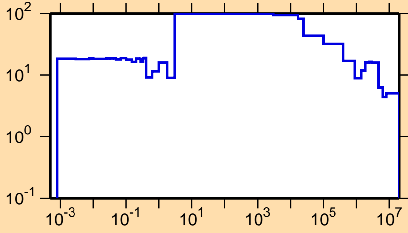
\Delta\sigma/\sigma vs. E for ^{130}\text{Pm}(n,el.)
