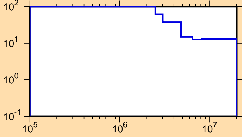
\Delta\sigma/\sigma vs. E for ^{130}\text{Pm}(n,n\text{cont.})
