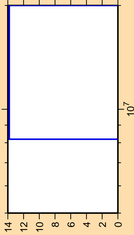
\Delta\sigma/\sigma vs. E for ^{130}\text{Pm}(n,2n\alpha)
