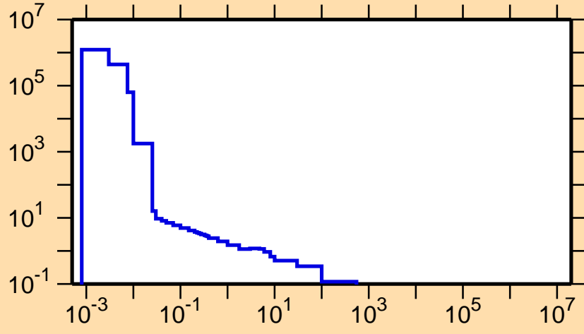
\sigma vs. E for ^{130}\text{Pm}(n,\alpha)
