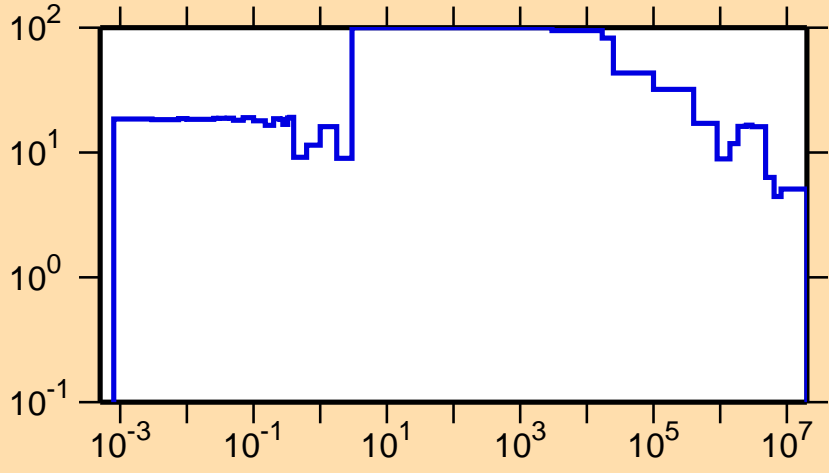
\Delta\sigma/\sigma vs. E for ^{130}\text{Pm}(n,\text{el.})
