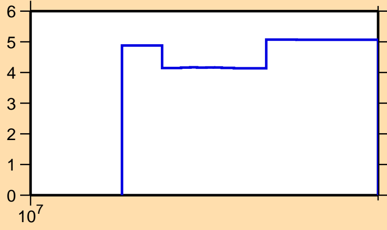
\Delta\sigma/\sigma vs. E for ^{131}\text{Pm}(n,el.)
