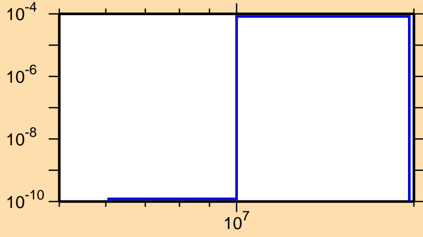
\sigma vs. E for ^{131}\text{Pm} (mt 45)
