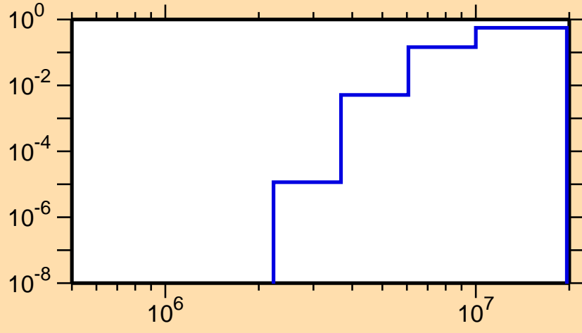
\sigma vs. E for ^{131}\text{Pm}(n,np)
