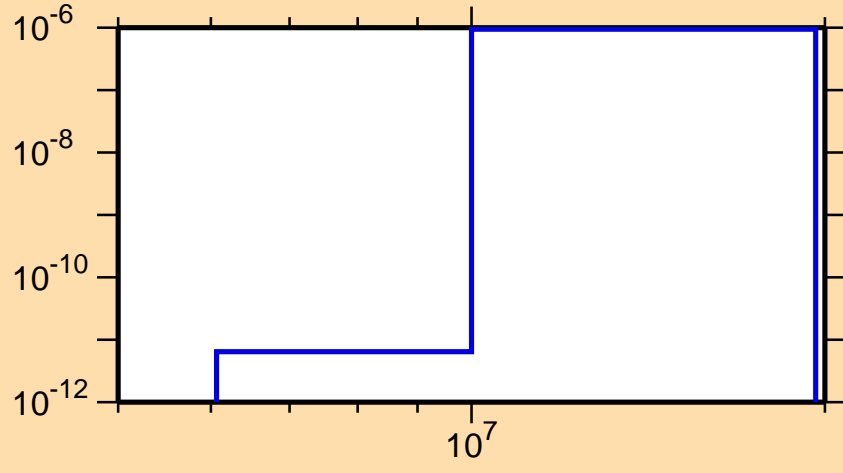
\sigma vs. E for ^{131}\text{Pm}(\text{mt117})
