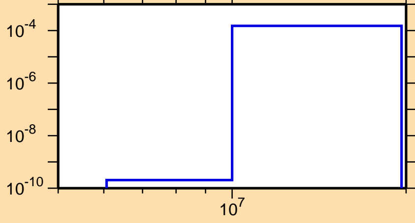
\sigma vs. E for ^{131}\text{Pm}(n,pd)
