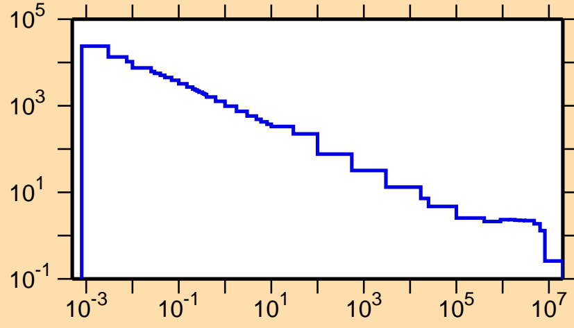
\sigma vs. E for ^{131}\text{Pm}(n,p)
