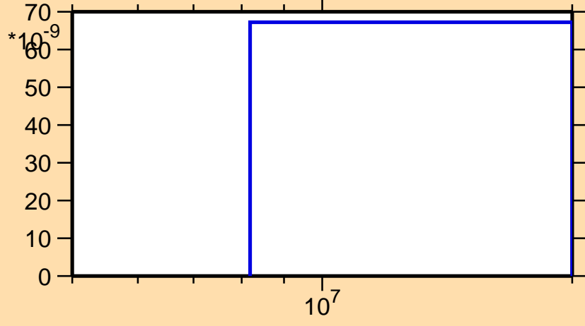
\sigma vs. E for ^{131}\text{Pm}(n,pt)
