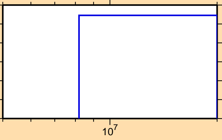
\sigma vs. E for ^{131}\text{Pm}(n,nd)
