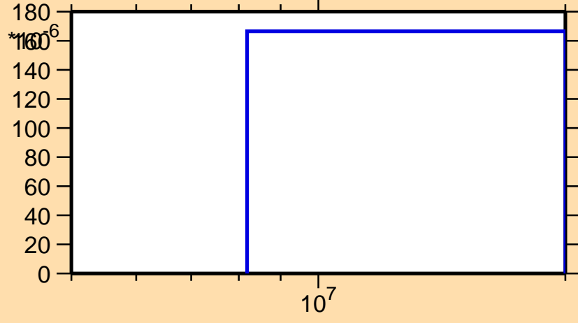
\sigma vs. E for ^{131}\text{Pm}(n,2n)
