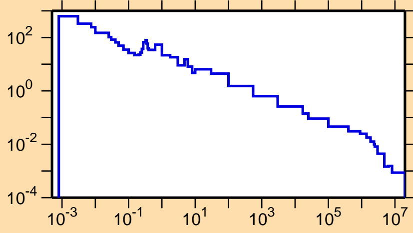
\sigma vs. E for ^{131}\text{Pm}(n,\gamma)
