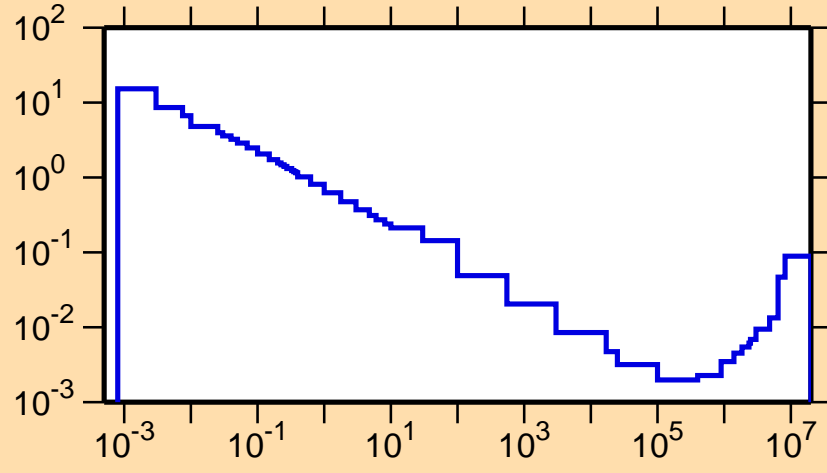
\sigma vs. E for ^{131}\text{Pm}(n,\alpha)
