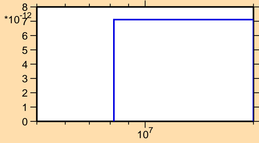
\sigma vs. E for ^{131}\text{Pm} (mt 34)
