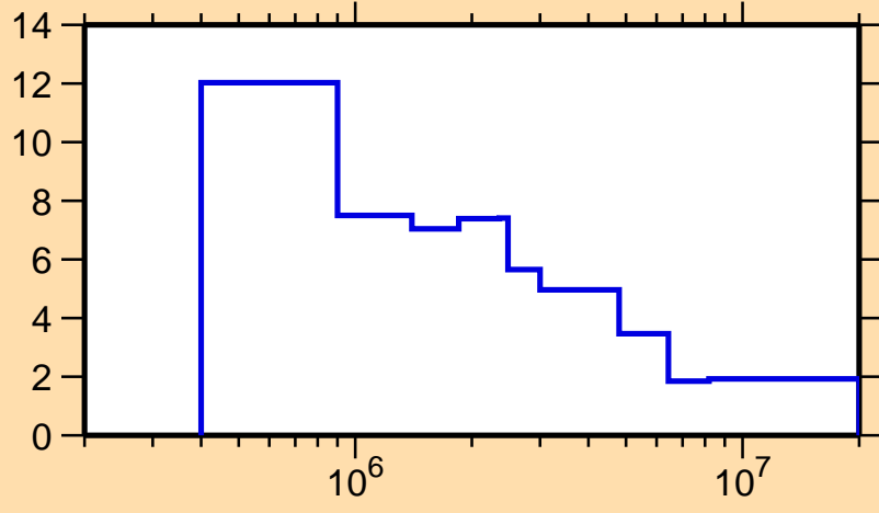
\Delta\sigma/\sigma vs. E for ^{131}\text{Pm}(n,\text{tot.})
