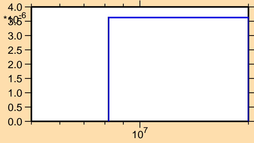
\sigma vs. E for ^{131}\text{Pm}(n,2np)
