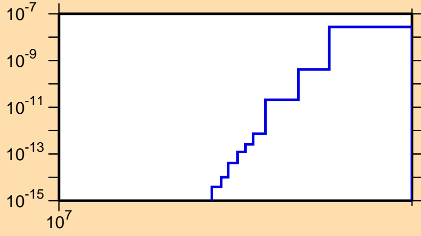
\sigma vs. E for ^{132}\text{Pm}(n,2n\alpha)
