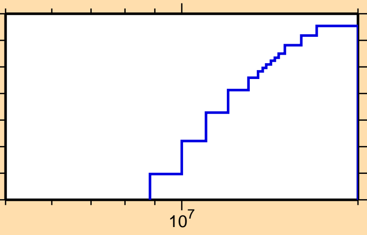
\sigma vs. E for ^{132}\text{Pm}(\text{mt117})
