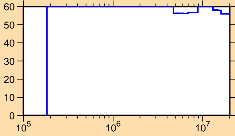
\Delta\sigma/\sigma vs. E for ^{132}\text{Pm}(n,n\text{cont.})
