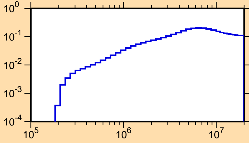
\sigma vs. E for ^{132}\text{Pm}(n,\text{inel.})
