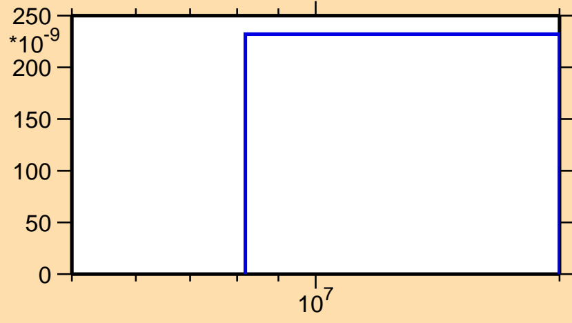
\sigma vs. E for ^{132}\text{Pm}(\text{mt117})
