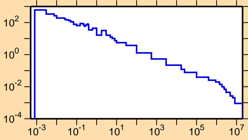
\sigma vs. E for ^{132}\text{Pm}(n,\gamma)
