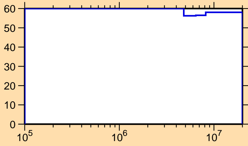
\Delta\sigma/\sigma vs. E for ^{132}\text{Pm}(n,ncont.)
