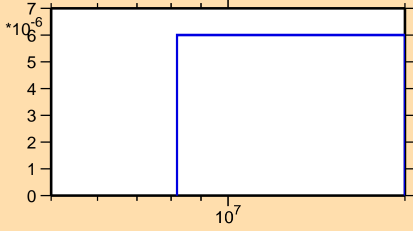
\sigma vs. E for ^{132}\text{Pm}(n,nd)
