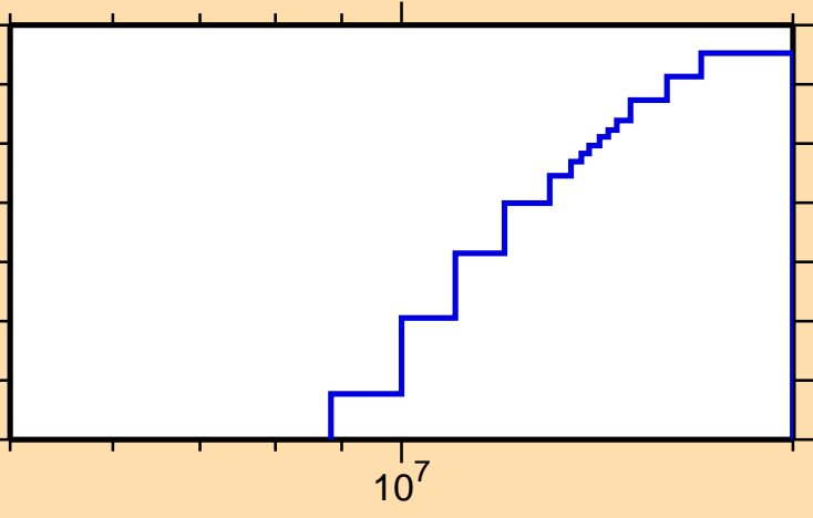
\sigma vs. E for ^{133}\text{Pm}(\text{mt117})
