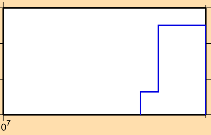
\sigma vs. E for ^{133}\text{Pm}(n,2n\alpha)
