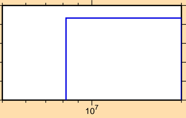
\sigma vs. E for ^{133}\text{Pm} (mt 34)
