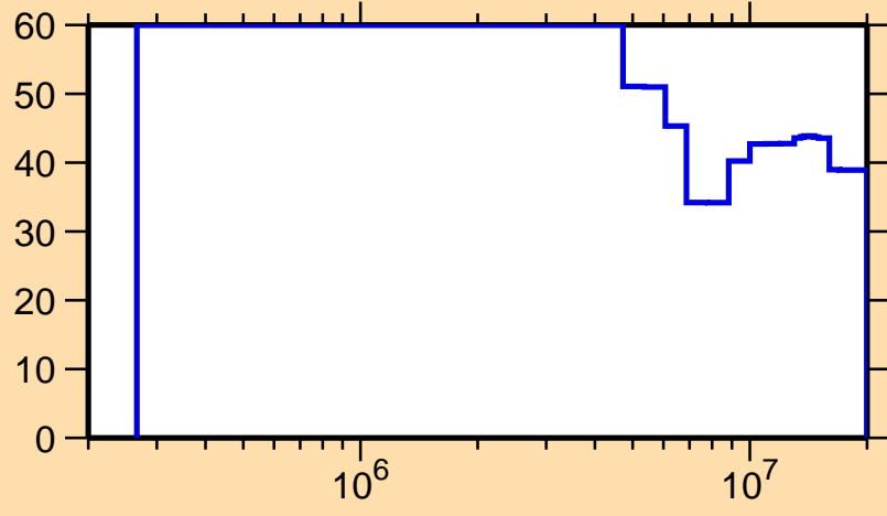
\Delta\sigma/\sigma vs. E for ^{133}\text{Pm}(n,n\text{cont.})
