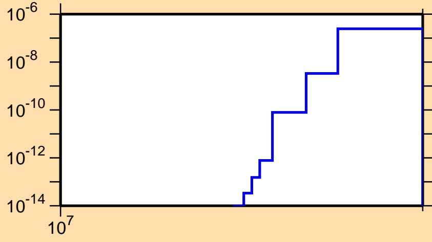
\sigma vs. E for ^{133}\text{Pm}(n,pt)
