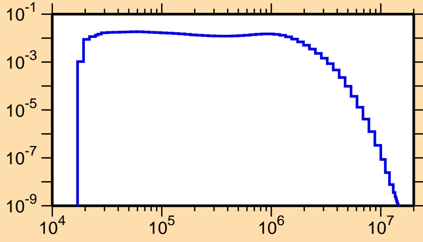
\sigma vs. E for ^{133}\text{Pm}(n,n_3)
