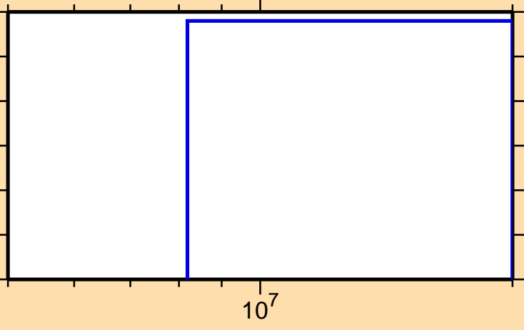
\sigma vs. E for ^{134}\text{Pm} (mt 34)
