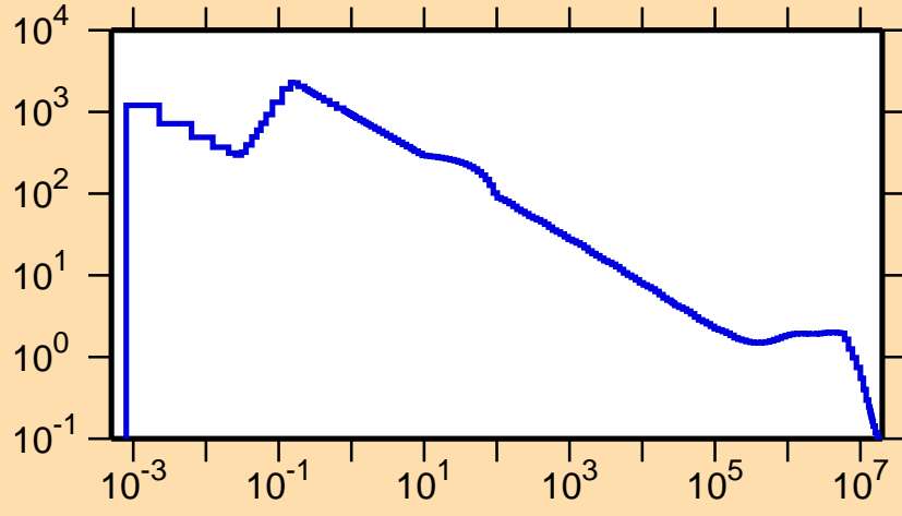
\sigma vs. E for ^{135}\text{Pm}(n,p)
