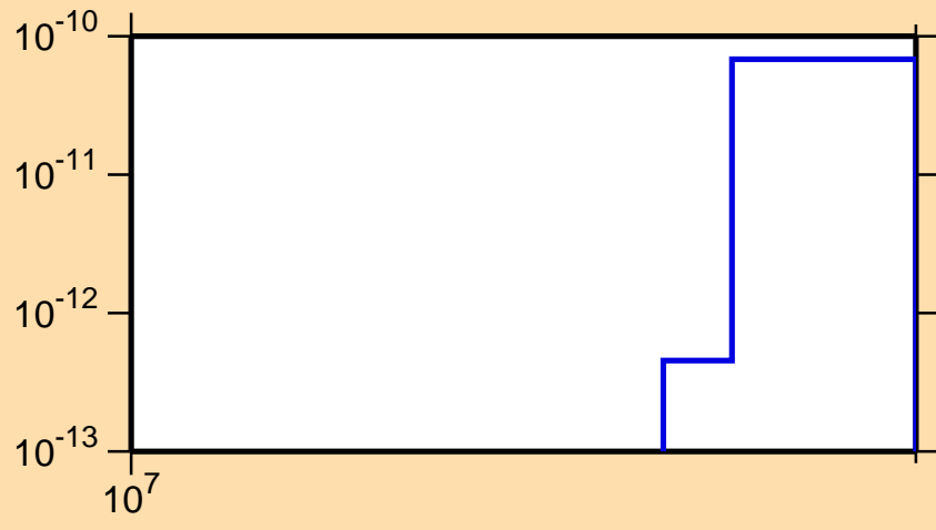
\sigma vs. E for ^{135}\text{Pm} (mt 34)
