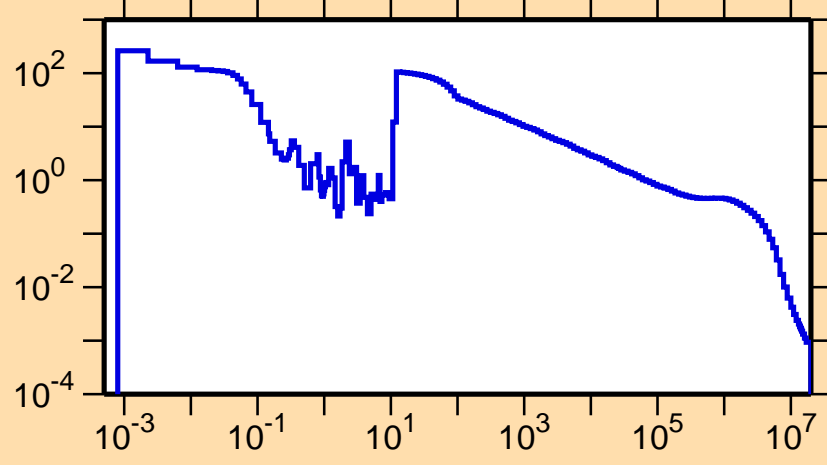
\sigma vs. E for ^{135}\text{Pm}(n,\gamma)
