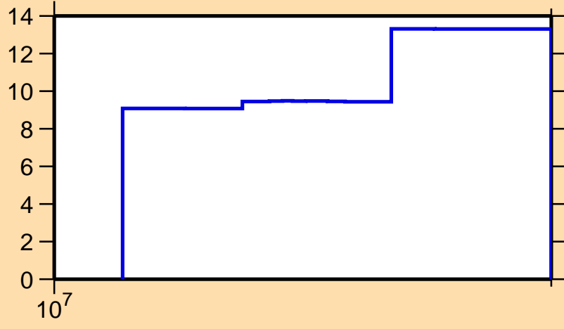
\Delta\sigma/\sigma vs. E for ^{135}\text{Pm}(n,\text{el.})
