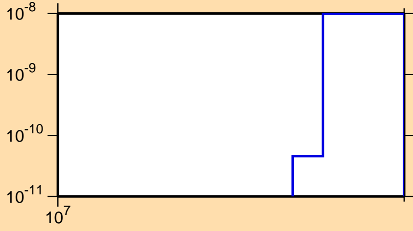
\sigma vs. E for ^{135}\text{Pm}(n,\text{pt})
