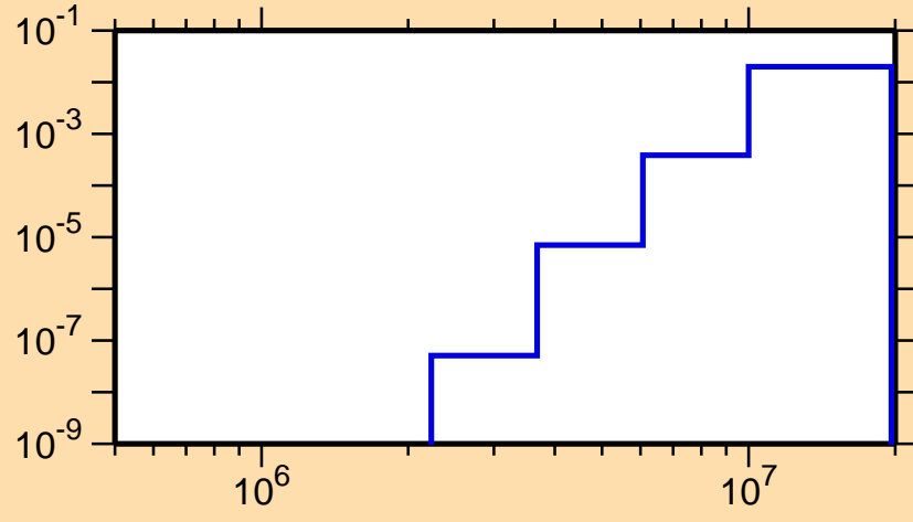
\sigma vs. E for ^{135}\text{Pm}(n,p\alpha)
