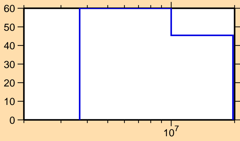
\Delta\sigma/\sigma vs. E for ^{135}\text{Pm}(n,n_1)
