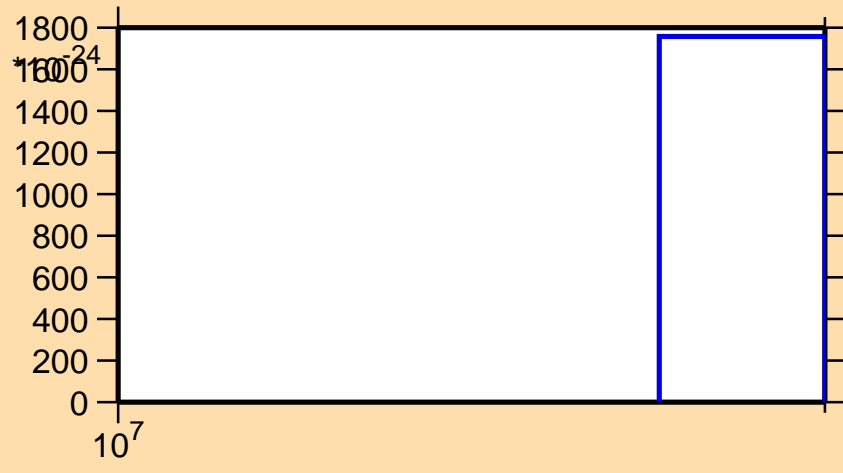
\sigma vs. E for ^{135}\text{Pm}(\text{mt } 11)
