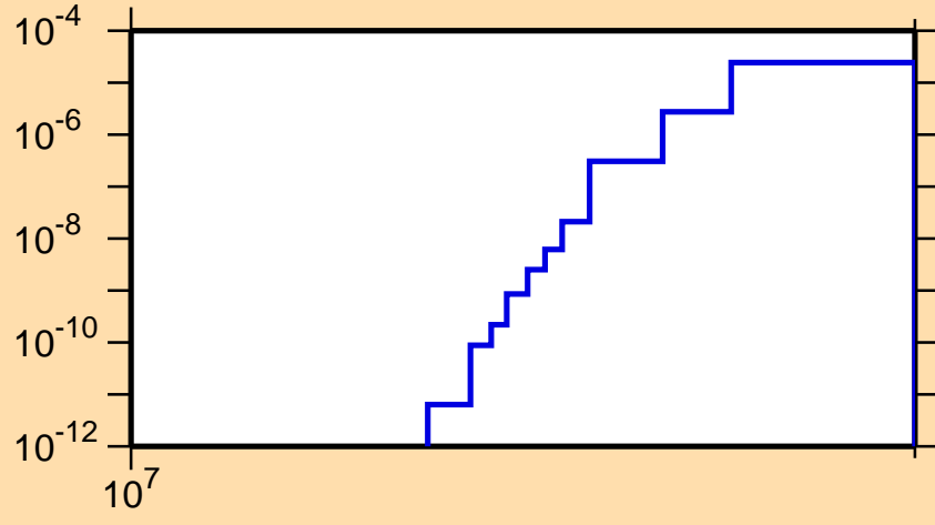
\sigma vs. E for ^{135}\text{Pm}(n,nd)
