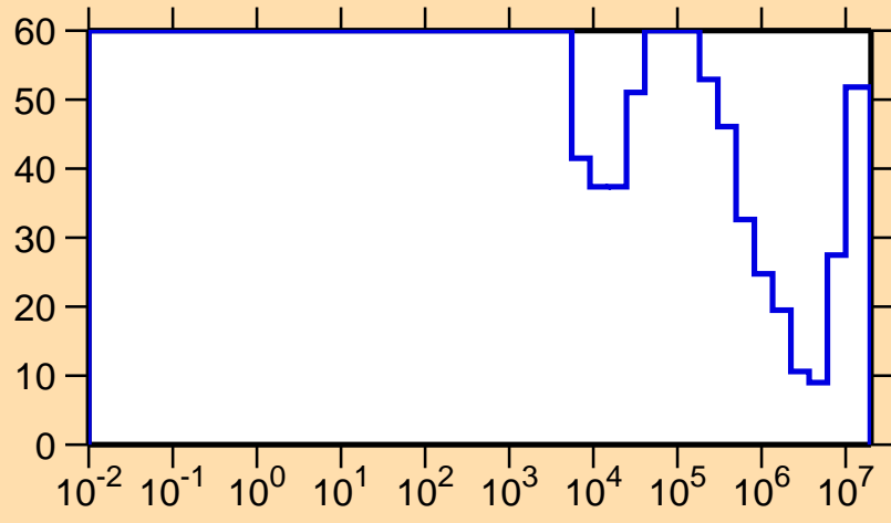
\Delta\sigma/\sigma vs. E for ^{135}\text{Pm}(n,p)
