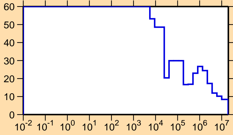
\Delta\sigma/\sigma vs. E for ^{135}\text{Pm}(n,\text{nonel.})
