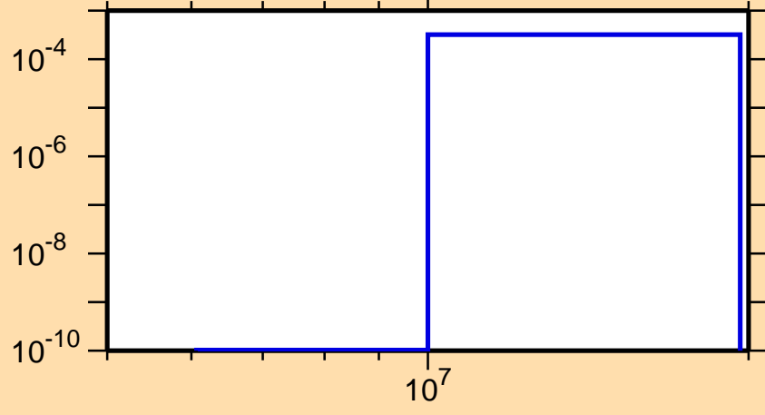
\sigma vs. E for ^{135}\text{Pm}(n,t)
