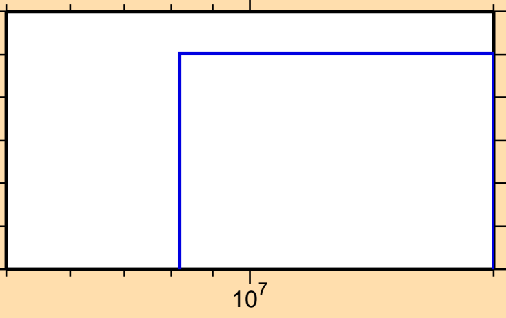
\sigma vs. E for ^{135}\text{Pm}(\text{mt117})
