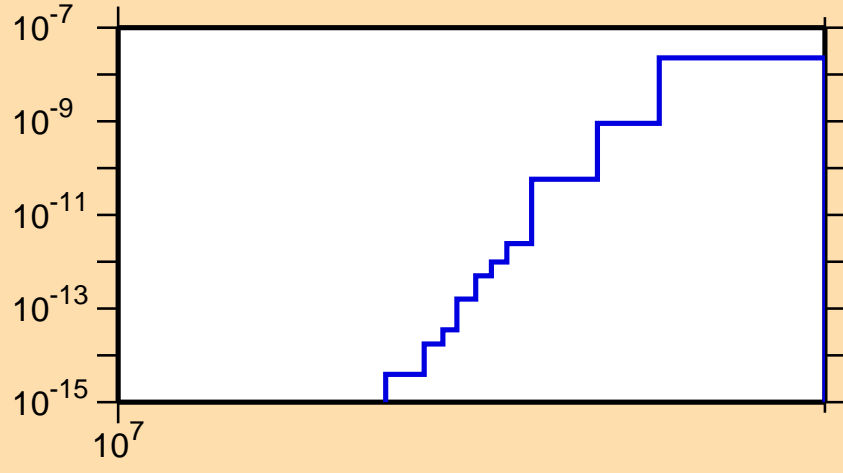
\sigma vs. E for ^{136}\text{Pm} (mt 34)
