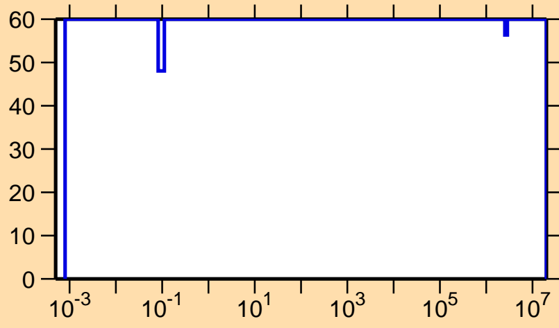
\Delta\sigma/\sigma vs. E for ^{136}\text{Pm}(n,\gamma)
