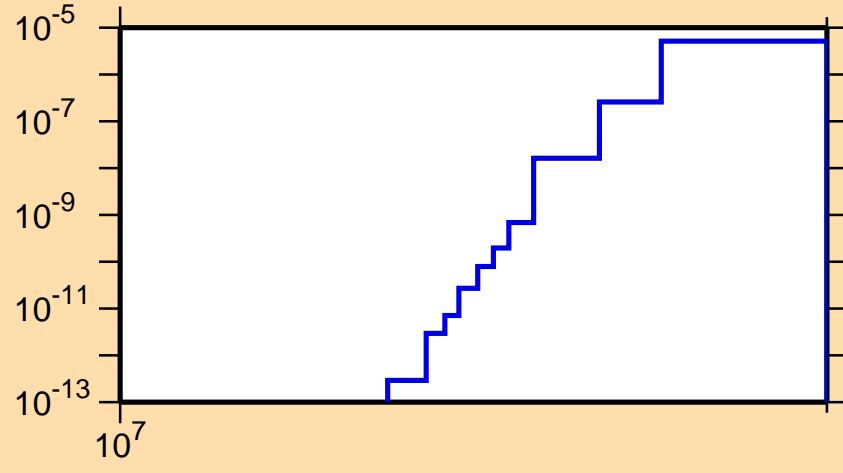
\sigma vs. E for ^{136}\text{Pm}(n,\text{pt})
