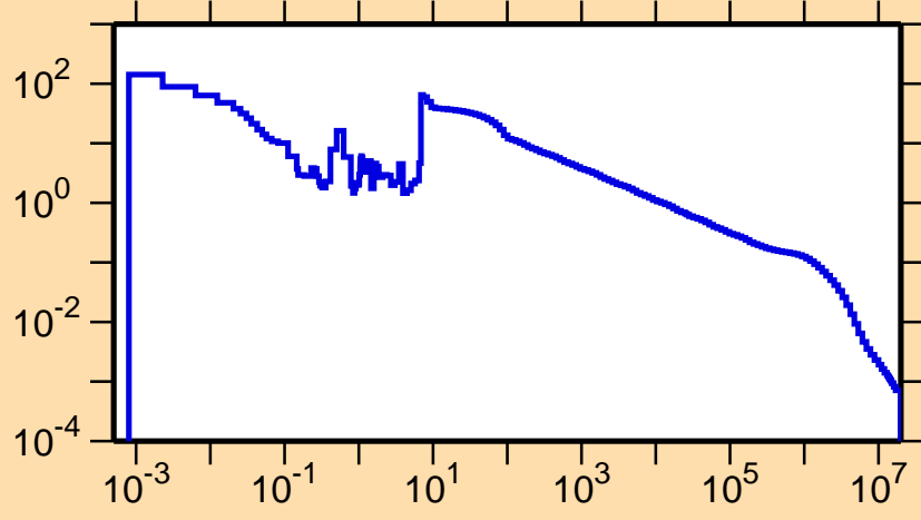
\sigma vs. E for ^{136}\text{Pm}(n,\gamma)
