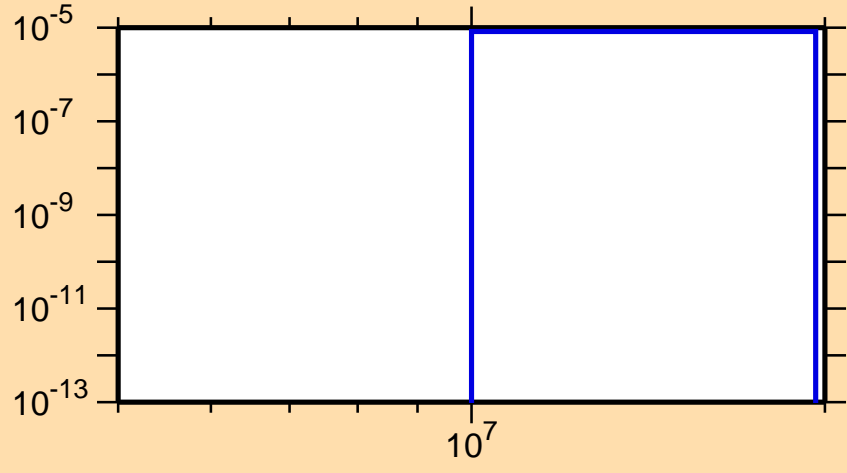
\sigma vs. E for ^{136}\text{Pm} (mt 45)
