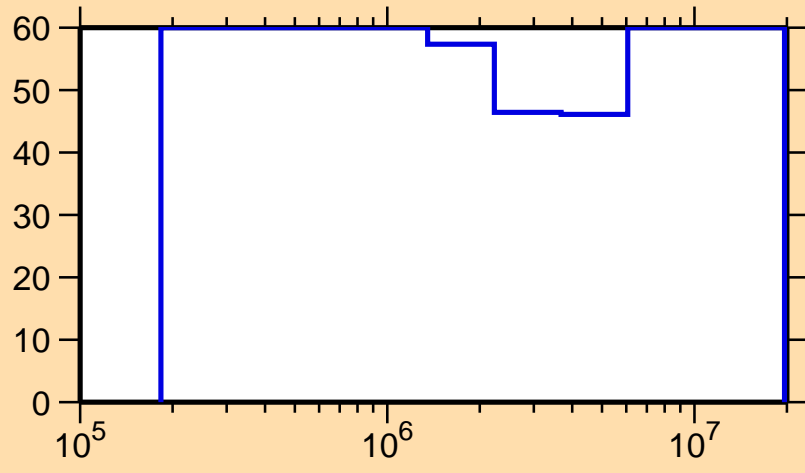
\Delta\sigma/\sigma vs. E for ^{136}\text{Pm}(n,ncont.)
