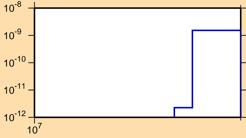
\sigma vs. E for ^{137}\text{Pm}(n,\text{pt})
